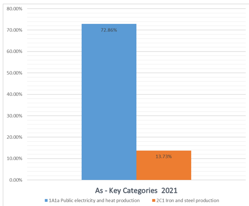
Figure 51. Key Categories assessments of As emissions for 2021
