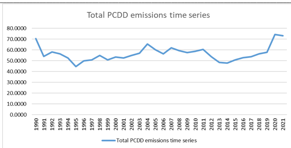
Figure 74. Total PCDD/PCDF emissions time series from 1990 to 2021.
