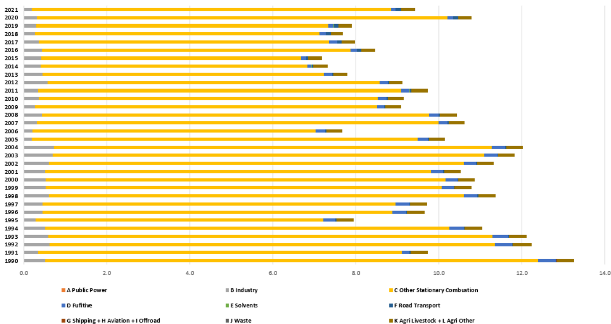
Figure 81. Distribution of benzo (b) fluoranthene between sectors for period 1990 – 2021.
