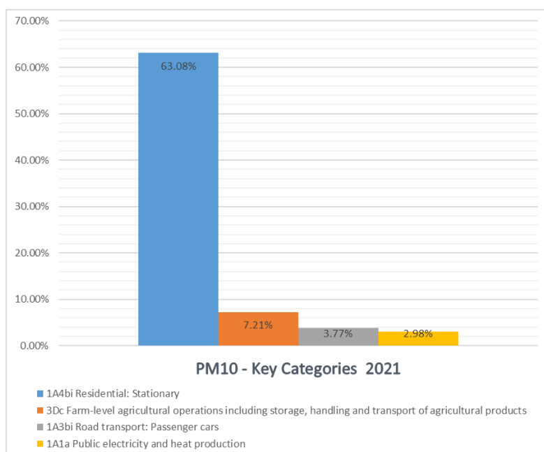
Figure 23. Key Categories assessments of PM10 emissions for 2021
