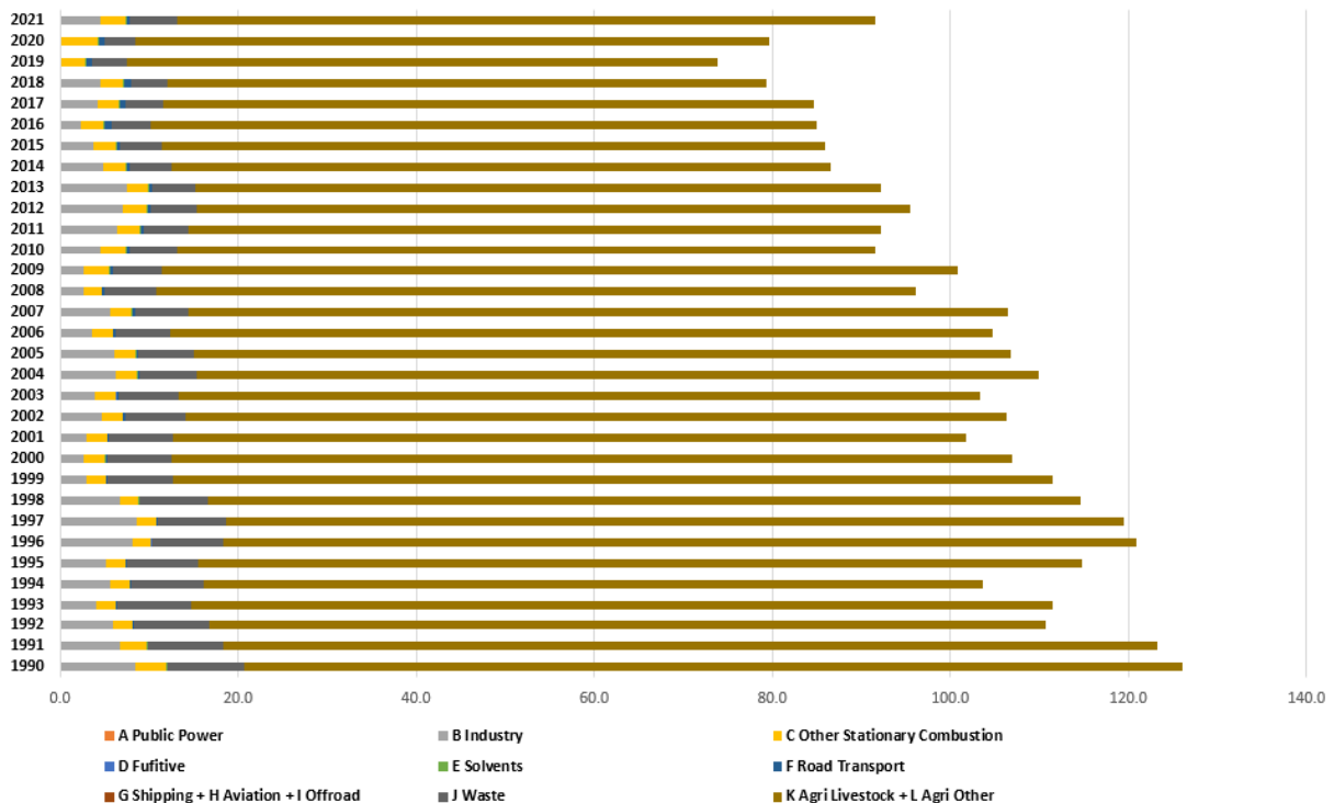
Figure 13. Distribution of NH 3 between sectors for period 1990 – 2021
