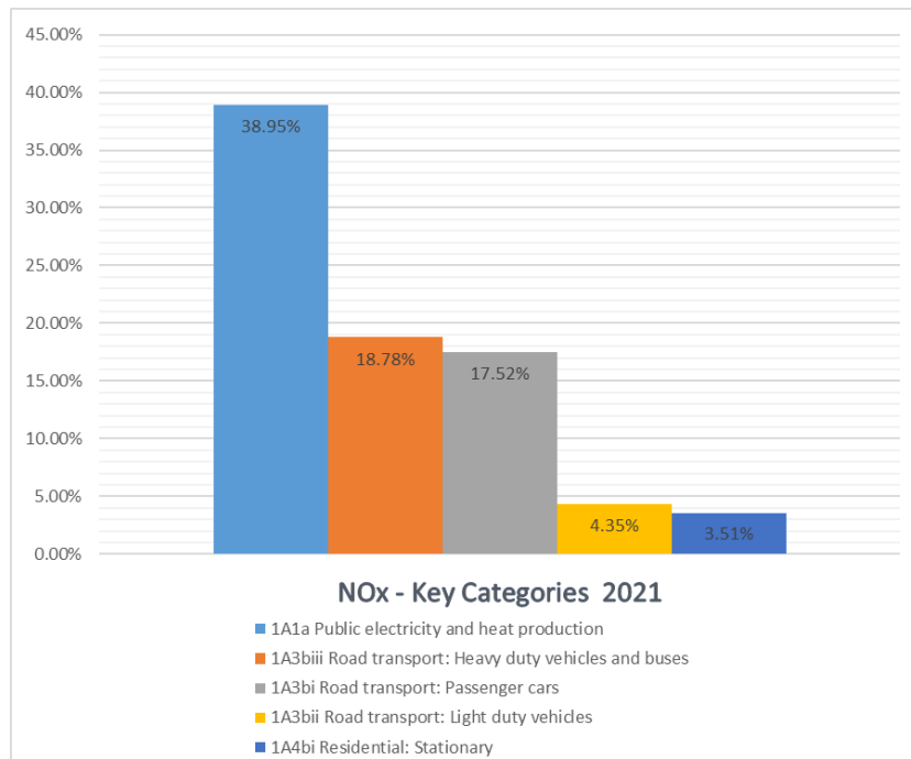
Figure 3. Key Categories assessments of NOx emissions for 2021
