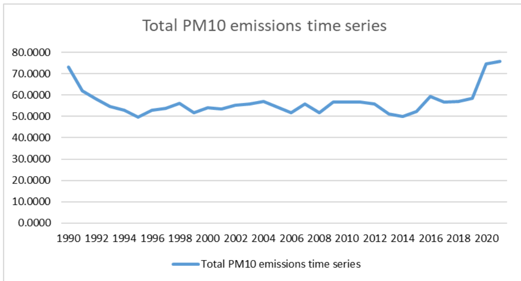
Figure 22. Total PM 10 emissions time series from 1990 to 2021.
