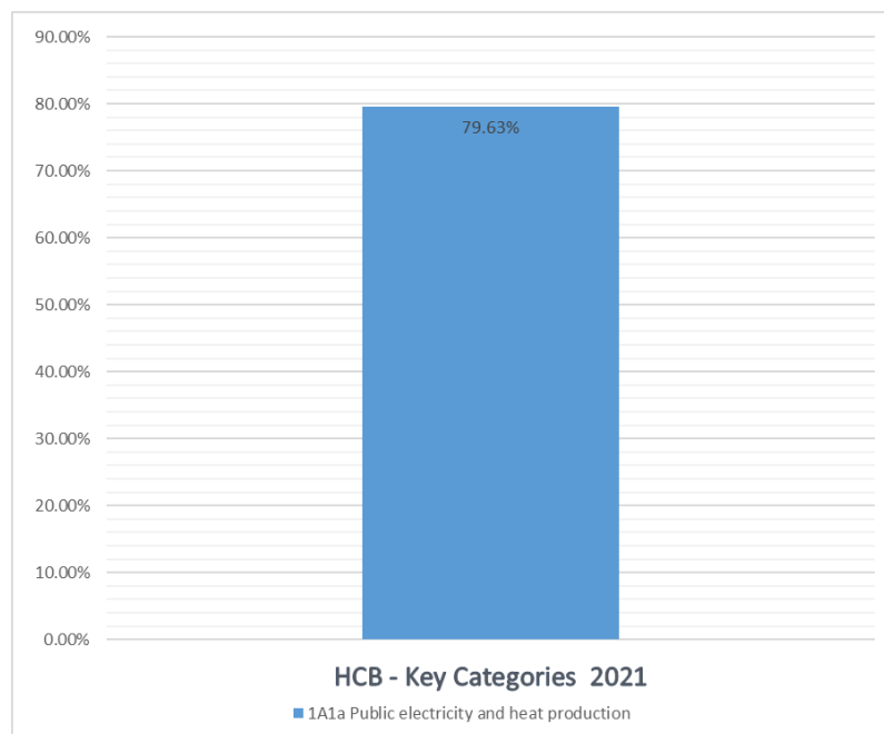
Figure 99. Key Categories assessments of HCB emissions for 2021.
