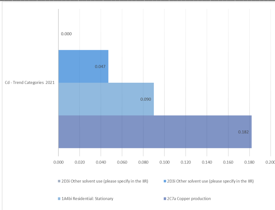
Figure 44. Trends assessments of Cd emissions for base year and 2021
