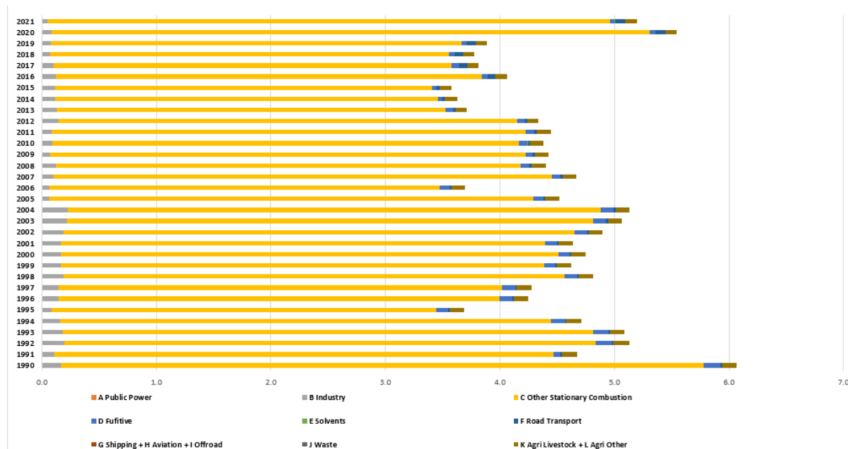
Figure 89. Distribution of Indeno (1,2,3-cd) pyrene between sectors for period 1990 – 2021.
