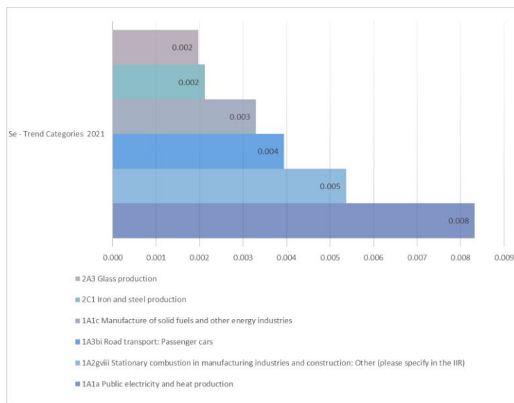
Figure 68. Trends assessments of Se emissions for base year and 2021
