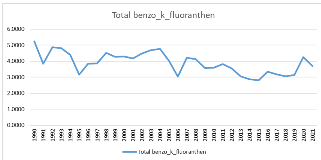
Figure 86. Total benzo k fluoranthen emissions time series from 1990 to 2021.
