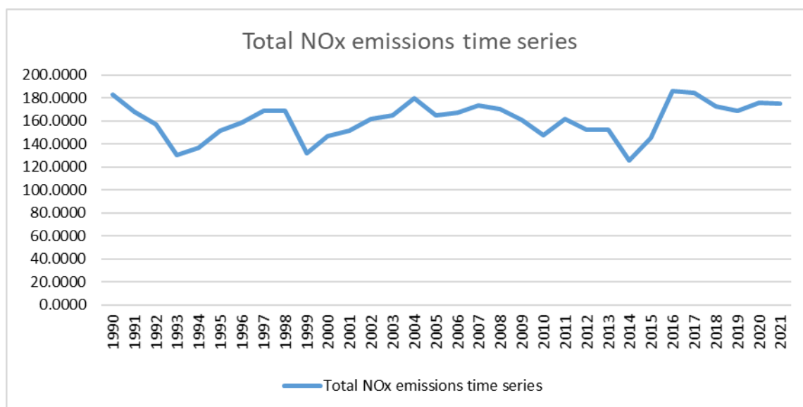
Figure 2. Total NOx emissions time series from 1990 to 2021.
