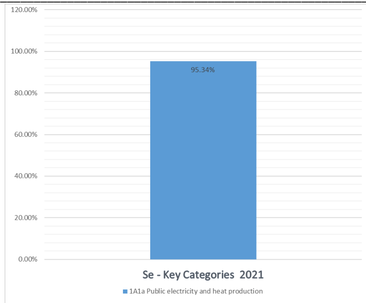
Figure 67. Key Categories assessments of Se emissions for 2021.
