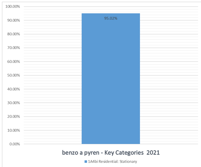
Figure 79. Key Categories assessments of benzo a pyren emissions for 2021.
