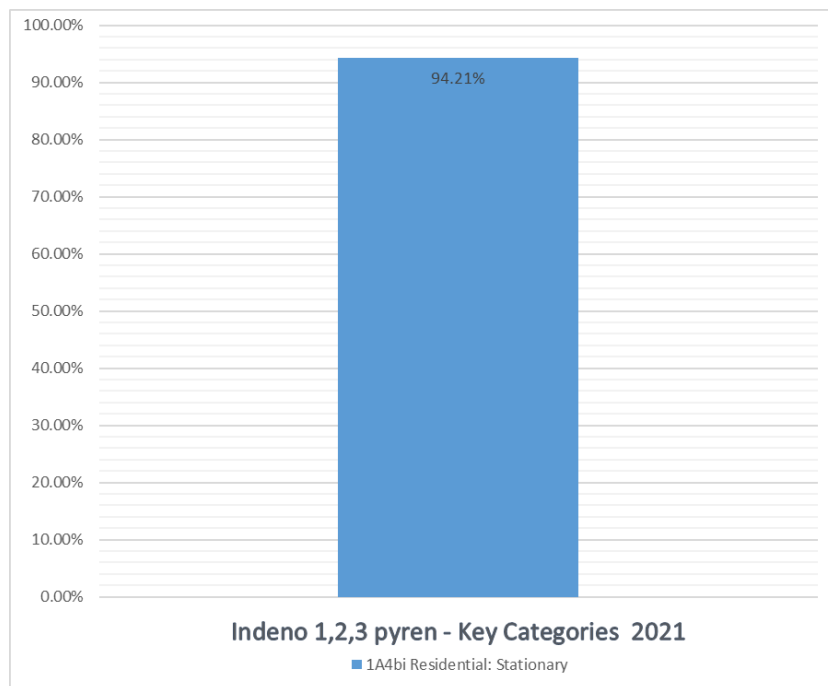
Figure 91. Key Categories assessments of Indeno 1,2,3 pyren emissions for 2021.
