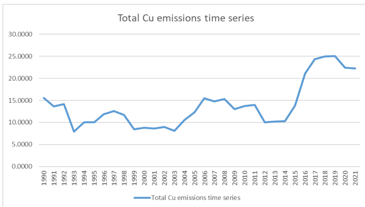
Figure 58. Total Cu emissions time series from 1990 to 2021.
