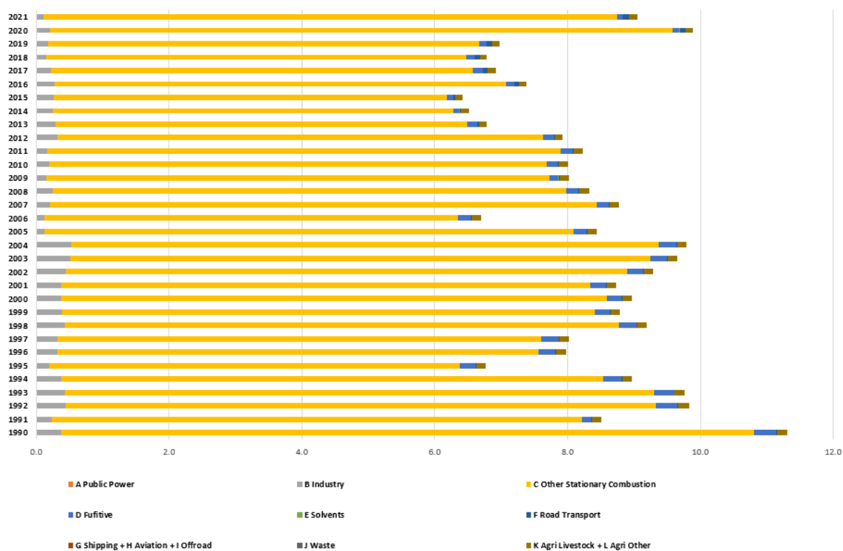
Figure 77. Distribution of Benzo (a) pyrene between sectors for period 1990 – 2021.
