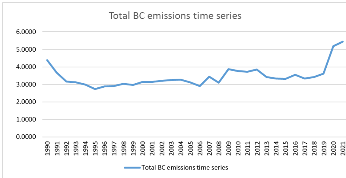
Figure 30. Total BC emissions time series from 1990 to 2021.
