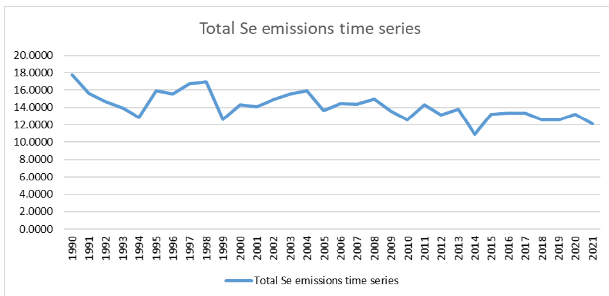
Figure 66.Total Se emissions time series from 1990 to 2021.
