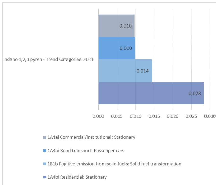
Figure 92. Trends assessments of Indeno 1,2,3 pyren emissions for base year and 2021
