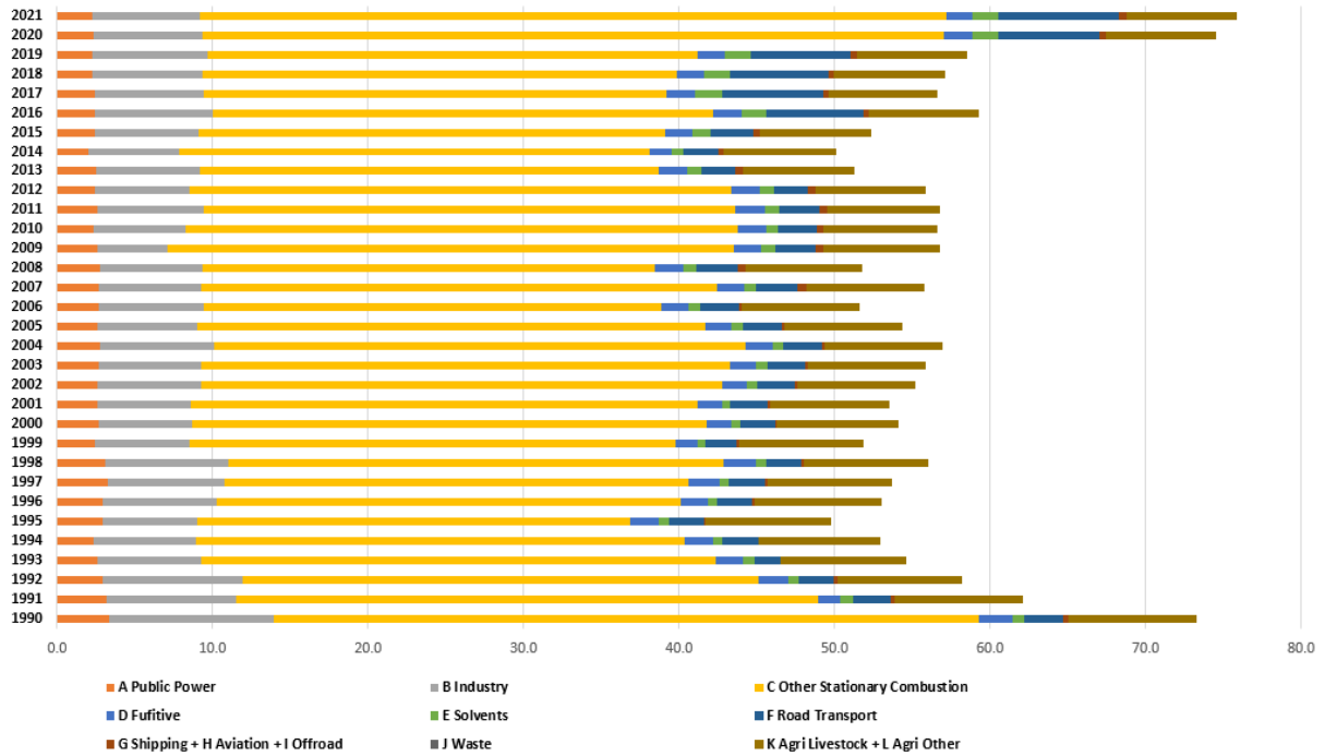
Figure 21. Distribution of PM 10 between sectors for period 1990 – 2021.
