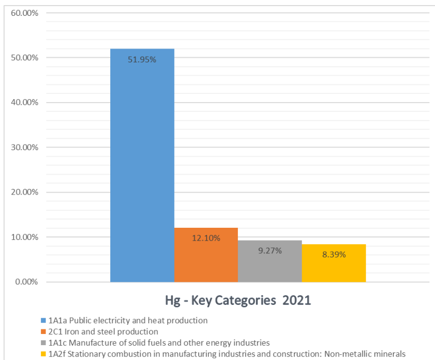
Figure 47. Key Categories assessments of Hg emissions for 2021.
