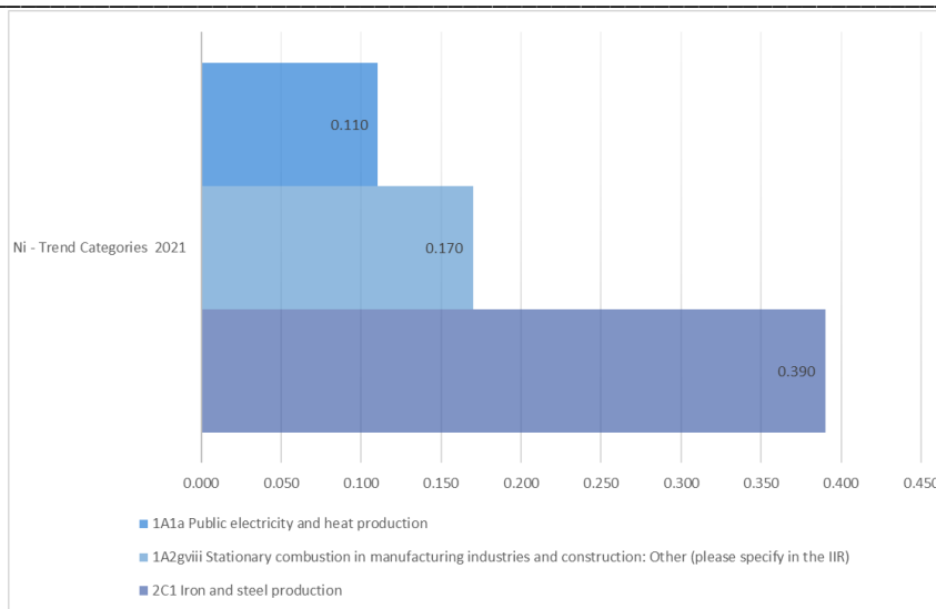
Figure 64. Trends assessments of Ni emissions for base year and 2021
