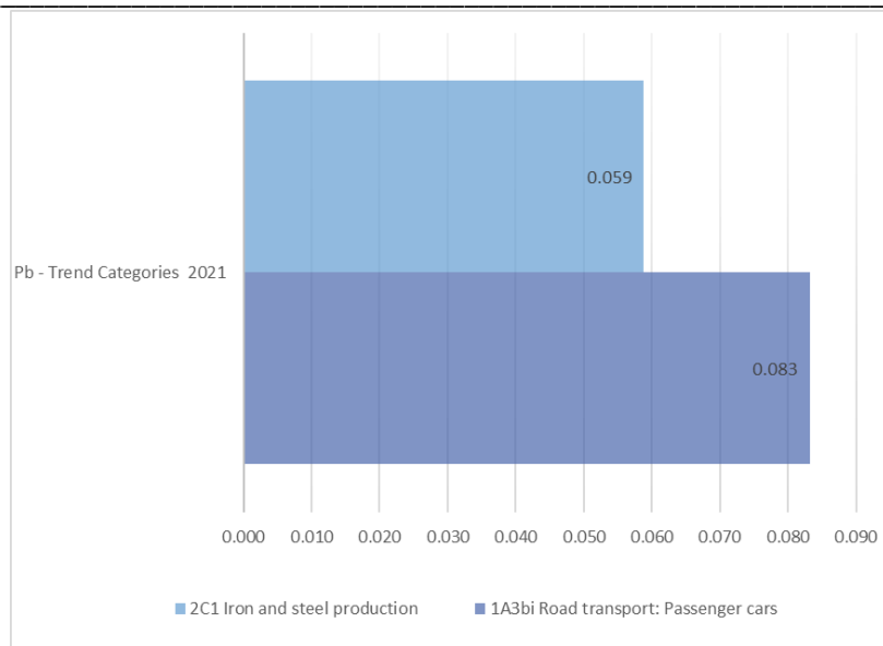
Figure 40. Trends assessments of Pb emissions for base year and 2021
