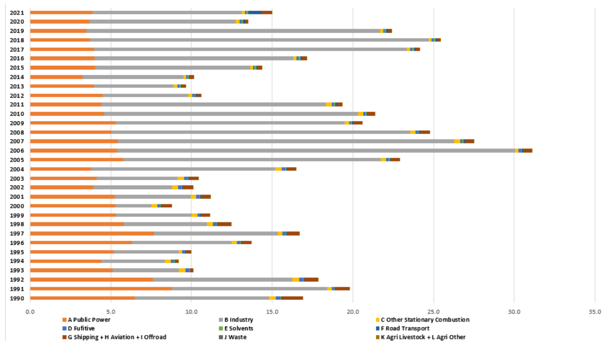
Figure 61. Distribution of Ni between sectors for period 1990 – 2021
