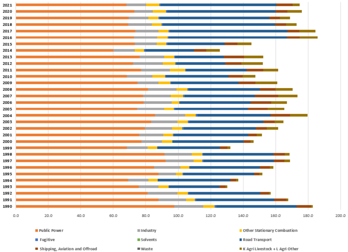
Figure 1. Distribution of NOx between sectors for period 1990 – 2021
