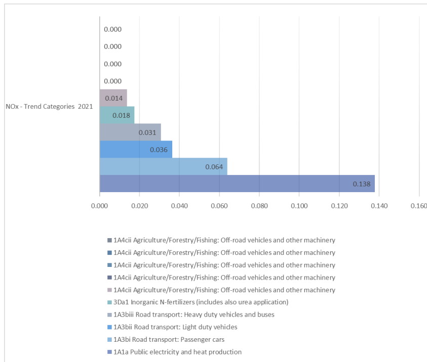
Figure 4. Trends assessments of NOx emissions for base year and 2021
