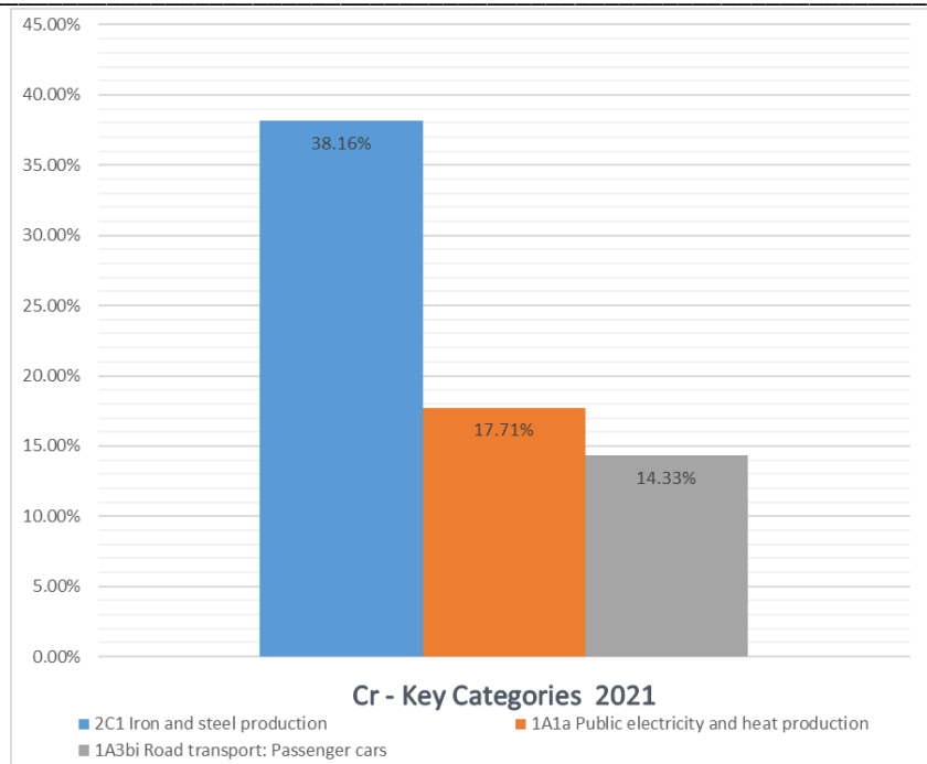
Figure 55. Key Categories assessments of Cr emissions for 2021.
