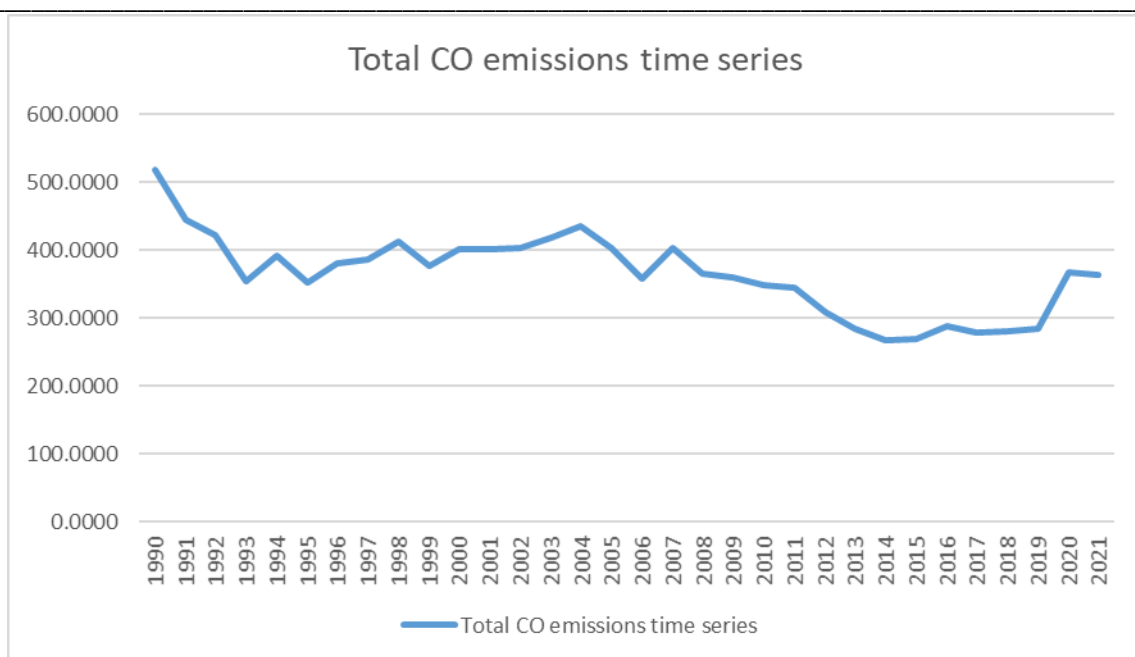
Figure 34. Total CO emissions time series from 1990 to 2021.
