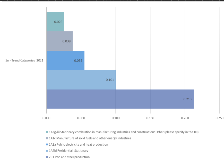
Figure 72. Trends assessments of Zn emissions for base year and 2021
