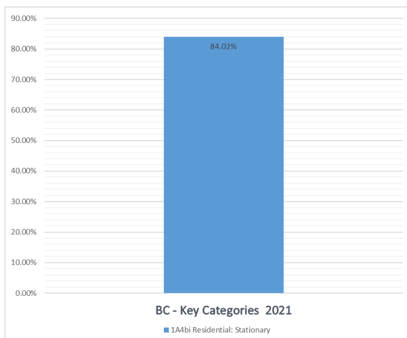
Figure 31. Key Categories assessments of BC emissions for 2021
