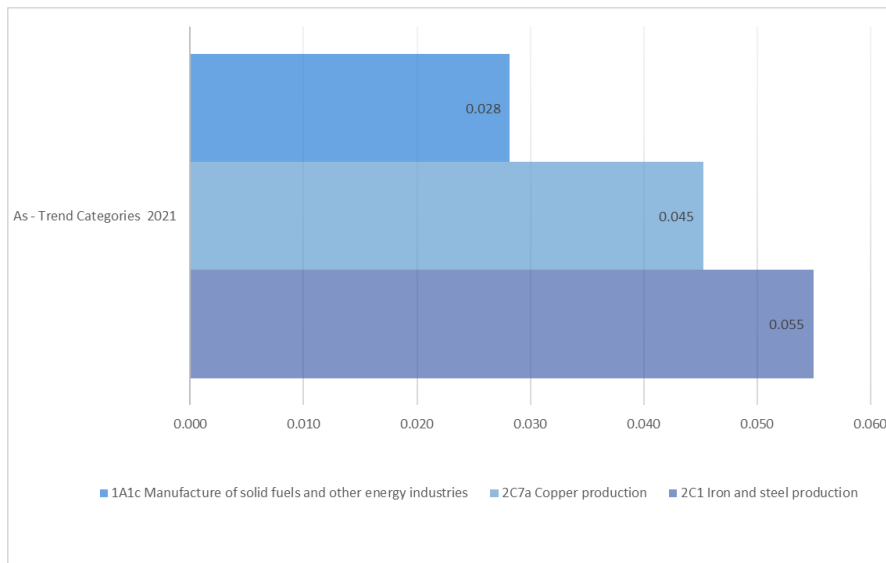
Figure 52. Trends assessments of As emissions for base year and 2021
