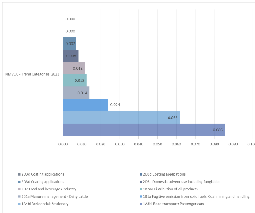
Figure 8. Trends assessments of NMVOC emissions for base year and 2021
