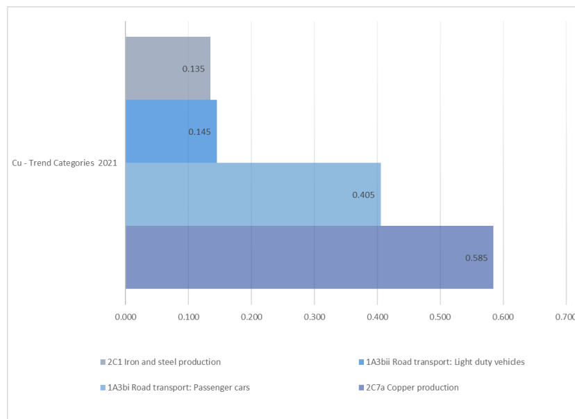
Figure 60. Trends assessments of Cu emissions for base year and 2021
