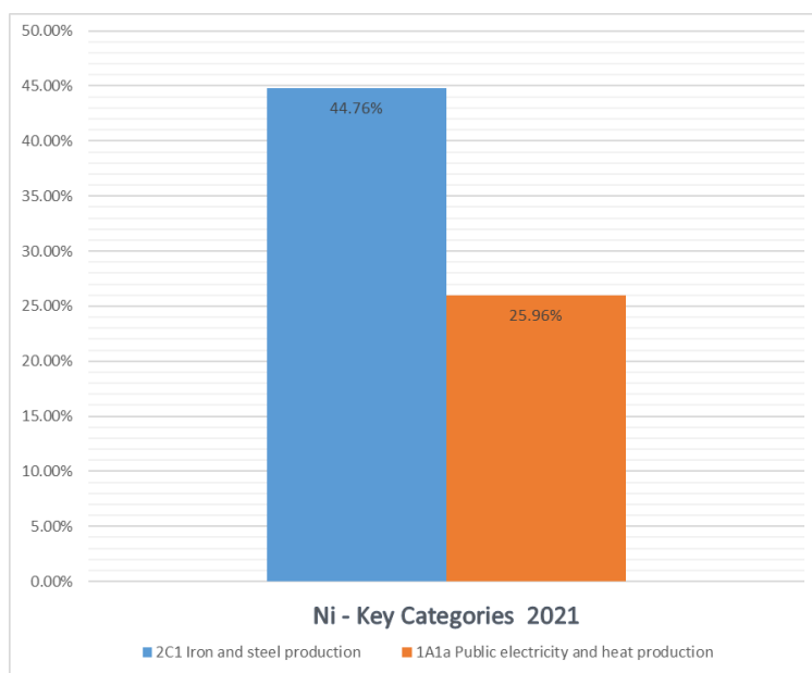
Figure 63. Key Categories assessments of Ni emissions for 2021
