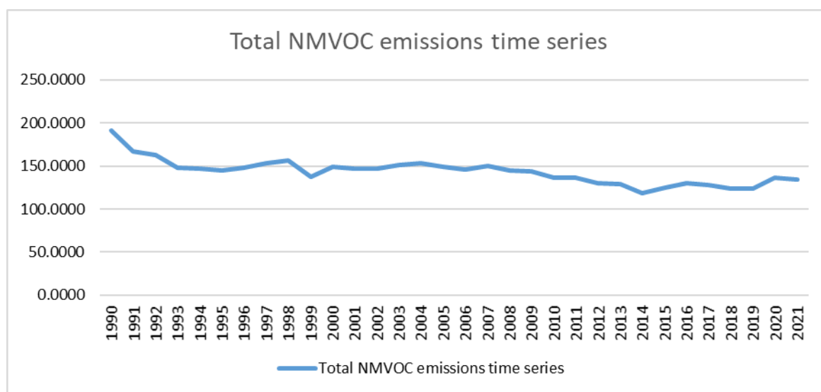
Figure 6. Total NMVOC emissions time series from 1990 to 2021.
