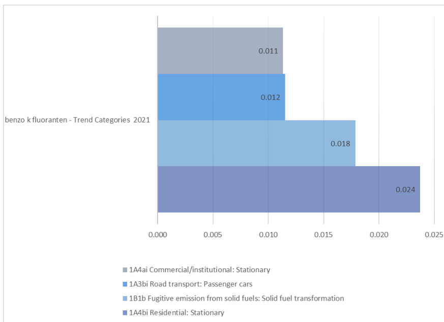
Figure 88. Trends assessments of benzo k fluoranthen emissions for base year and 2021
