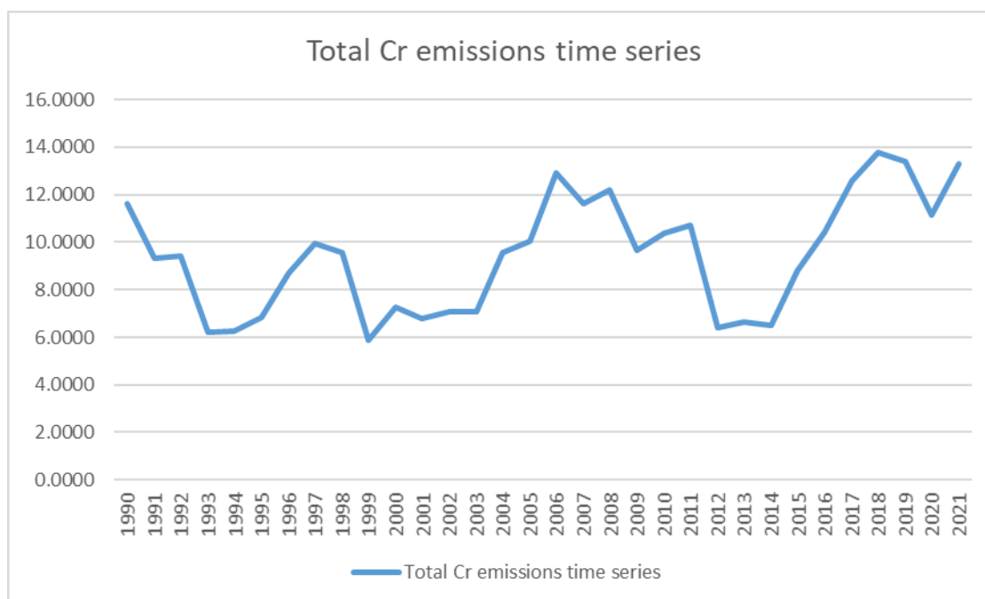
Figure 54. Total Cr emissions time series from 1990 to 2021.
