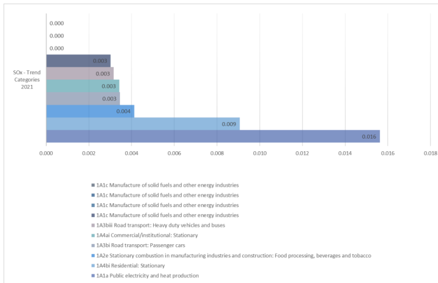
Figure 12. Trends assessments of SOx emissions for base year and 2021
