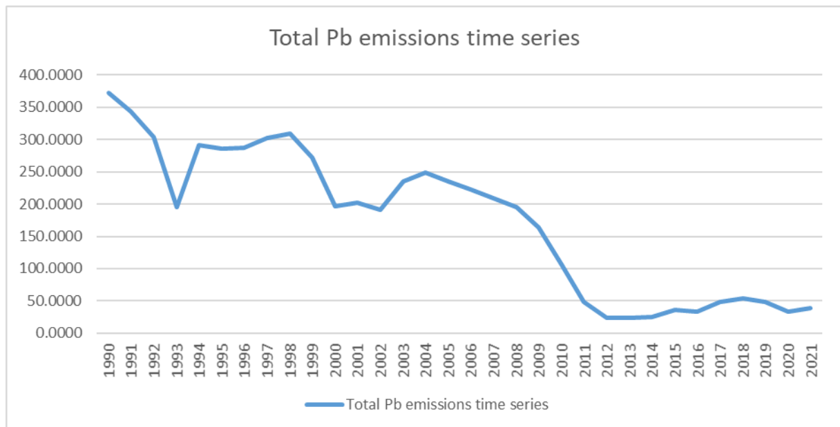
Figure 38. Total Pb emissions time series from 1990 to 2021.
