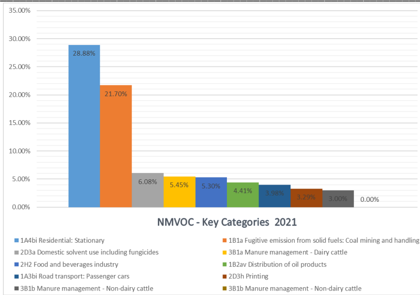
Figure 7. Key Categories assessments of NMVOC emissions for 2021
