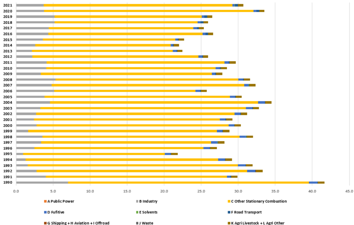
Figure 93. Distribution of Total 1-4 PAH between sectors for period 1990 – 2021.
