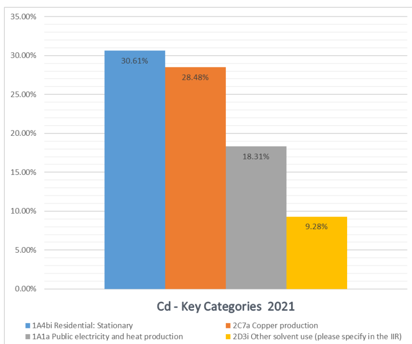
Figure 43. Key Categories assessments of Cd emissions for 2021.
