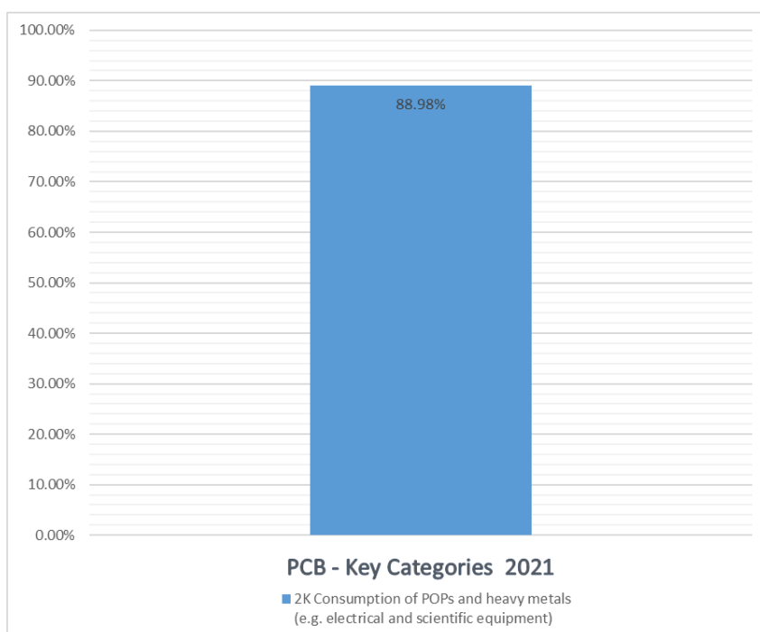
Figure 103. Key Categories assessments of PCB emissions for 2021.
