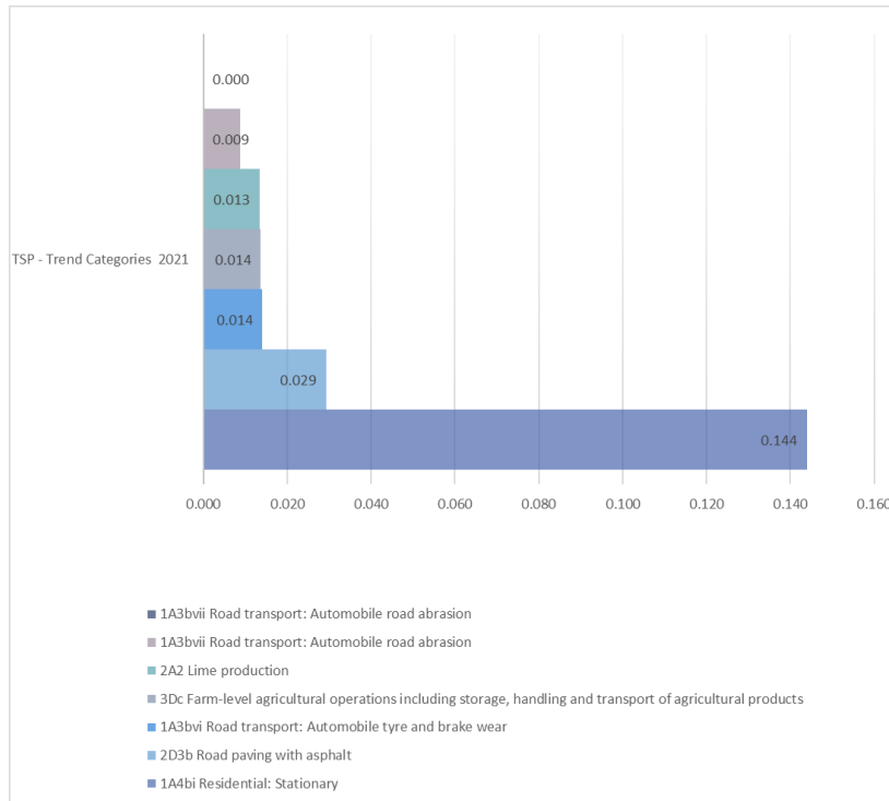
Figure 28. Trends assessments of TSP emissions for base year and 2021
