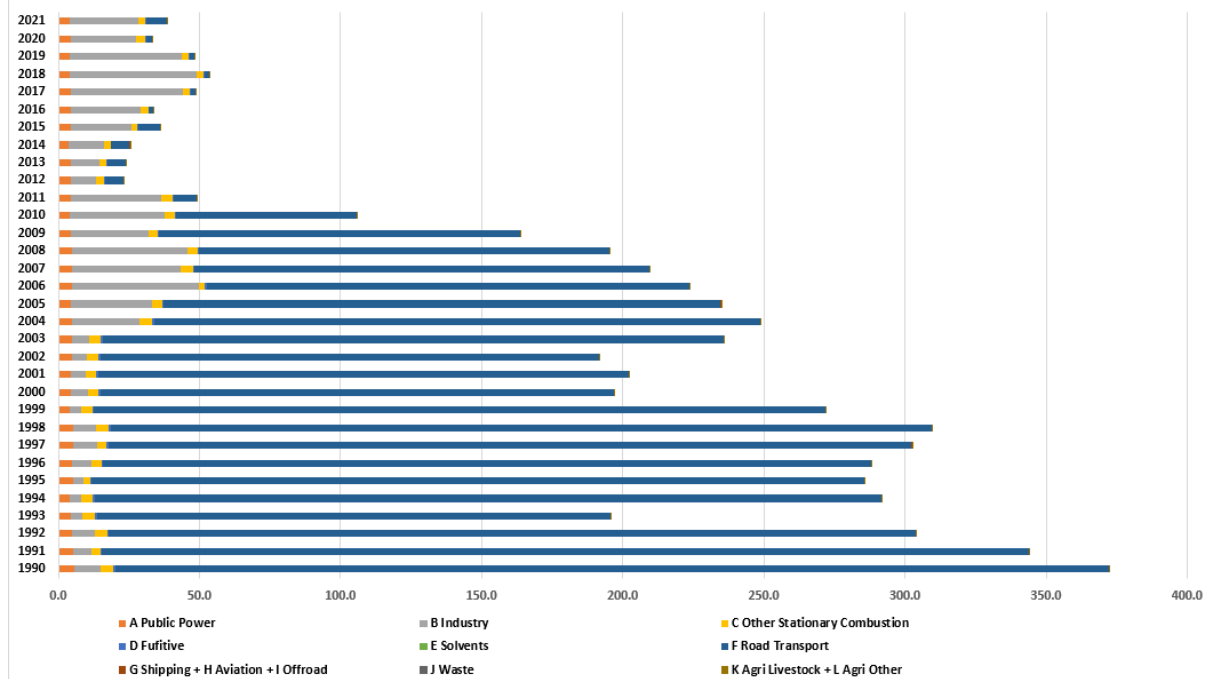
Figure 37. Distribution of Pb between sectors for period 1990 - 2021
