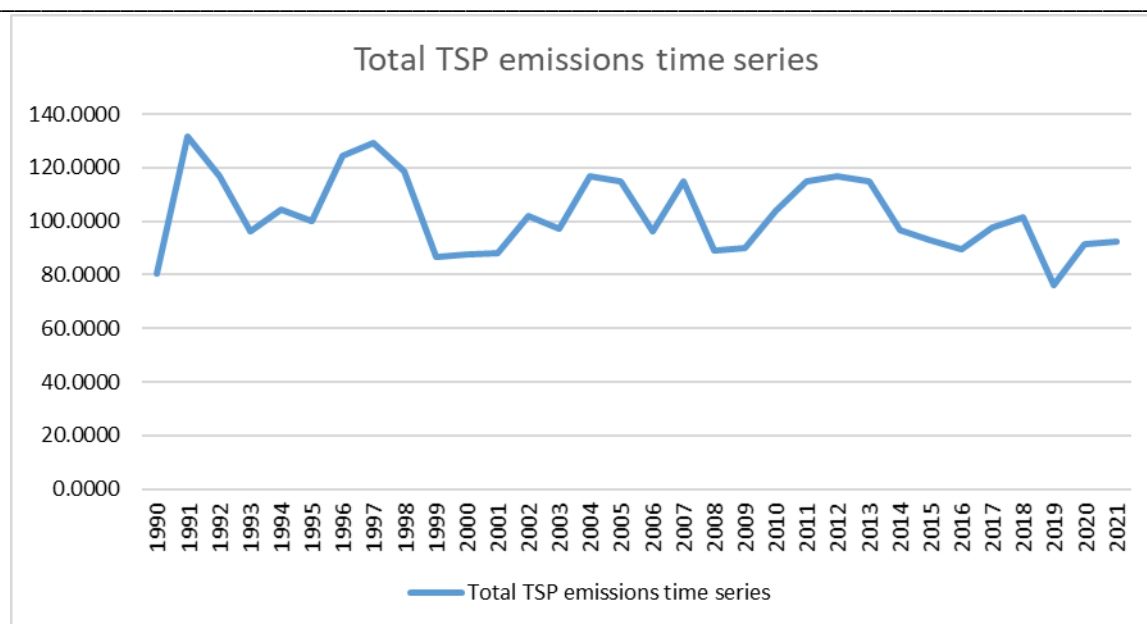
Figure 26. Total TSP emissions time series from 1990 to 2021.
