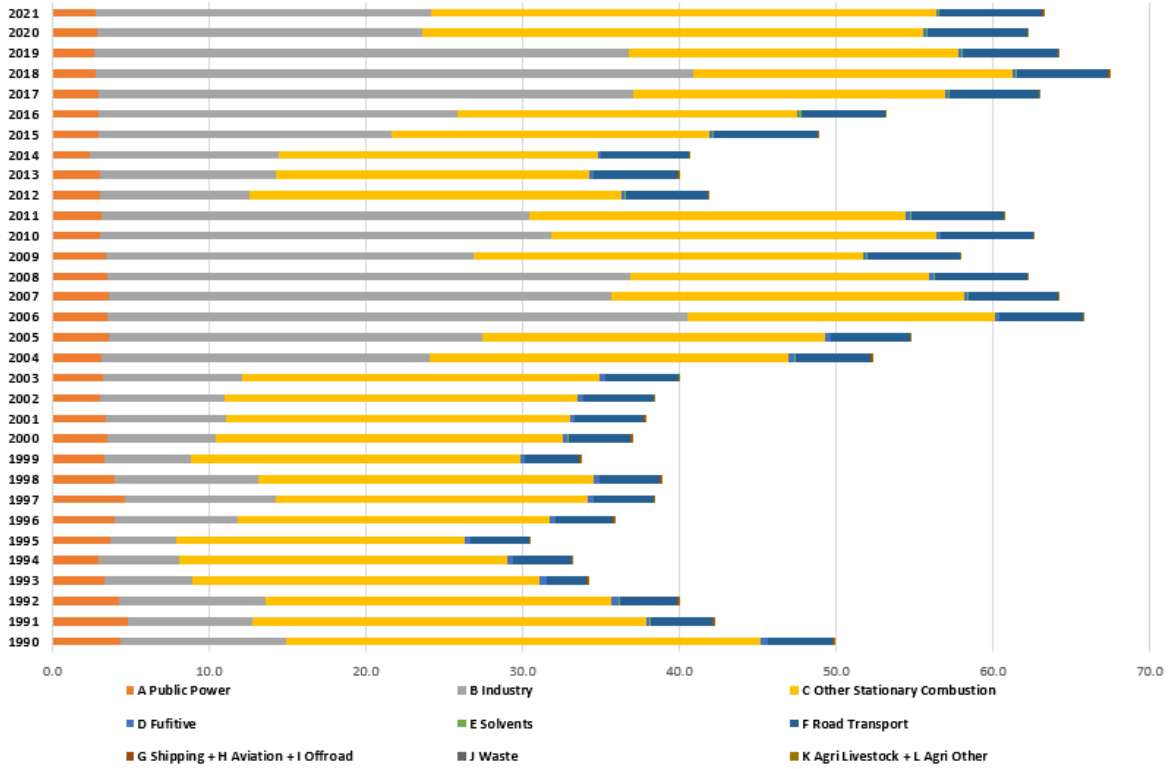
Figure 69. Distribution of Zn between sectors for period 1990 - 2021
