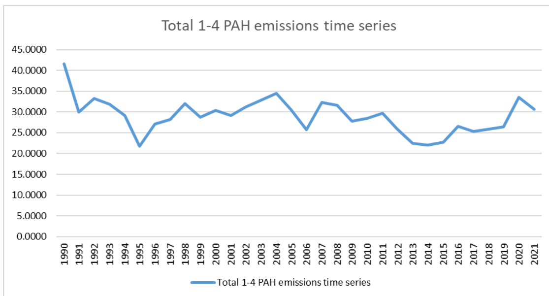
Figure 94. Total 1-4 PAH emissions time series from 1990 to 2021.
