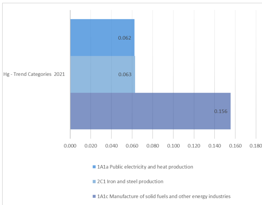
Figure 47. Key Categories assessments of Hg emissions for 2021.
