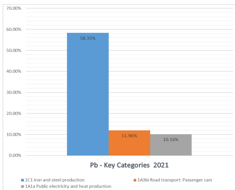
Figure 39. Key Categories assessments of Pb emissions for 2021.
