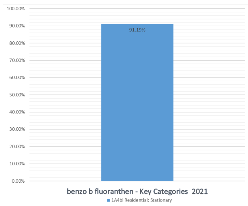
Figure 83. Key Categories assessments of benzo b fluoranthen emissions for 2021.
