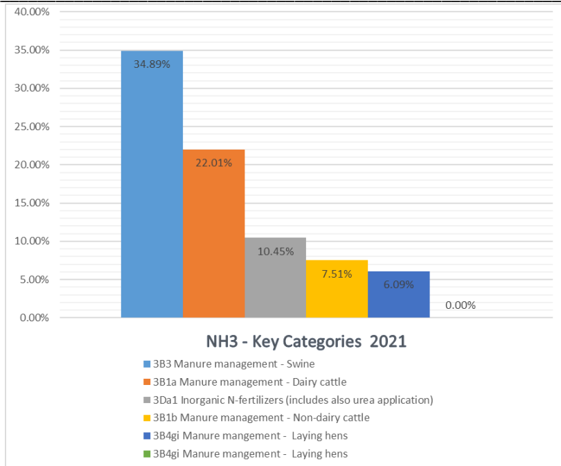
Figure 15. Key Categories assessments of NH3 emissions for 2021
