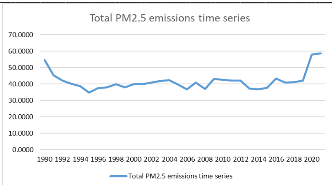
Figure 18. Total PM 2.5 emissions time series from 1990 to 2021.
