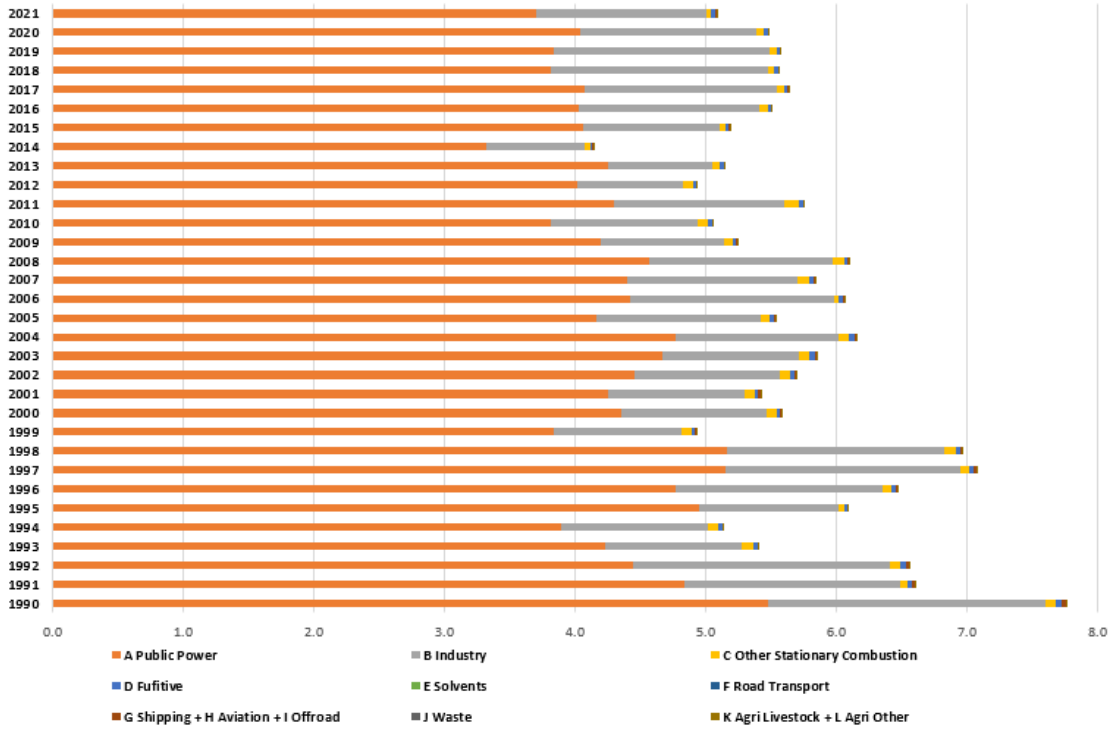
Figure 49. Distribution of As between sectors for period 1990 – 2021.
