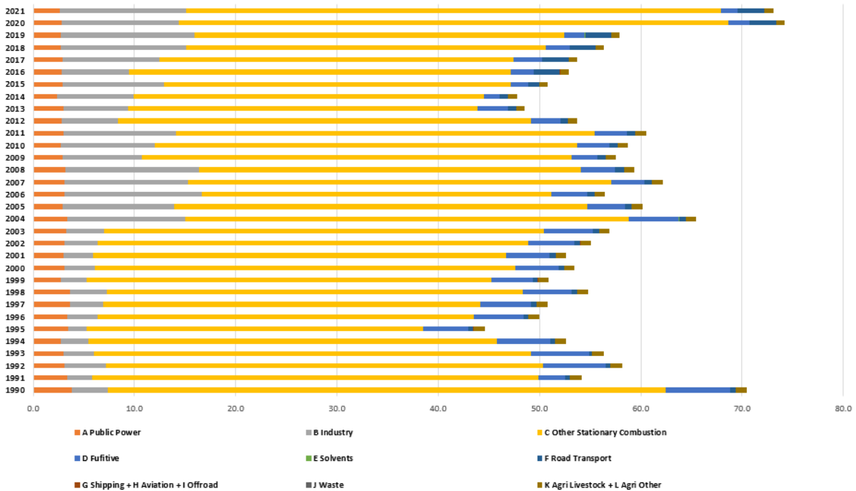
Figure 73. Distribution of PCDD/PCDF between sectors for period 1990 – 2021
