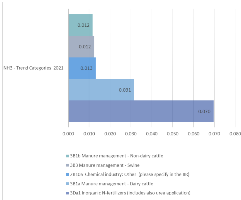
Figure 16. Trends assessments of NH3 emissions for base year and 2021
