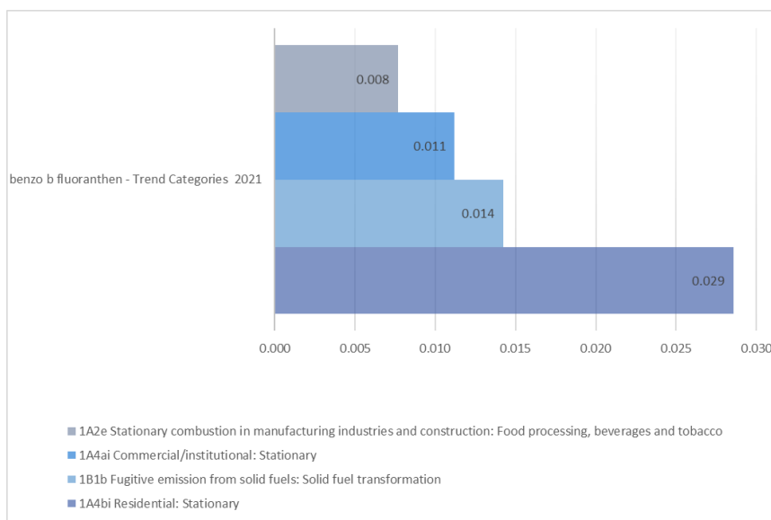
Figure 84. Trends assessments of benzo b fluoranthen emissions for base year and 2021
