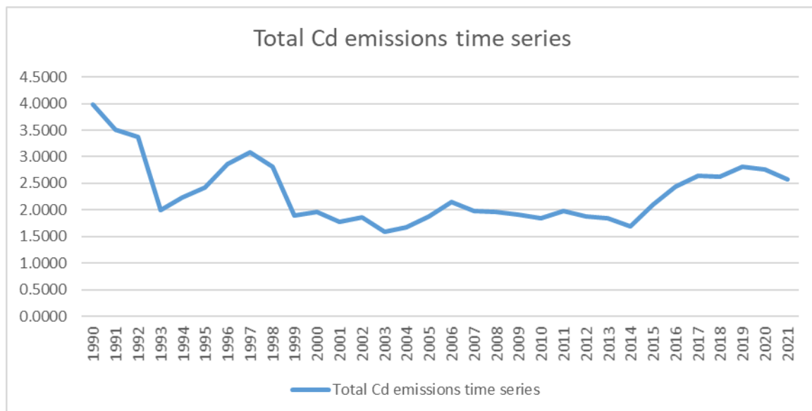
Figure 42. Total Cd emissions time series from 1990 to 2021.
