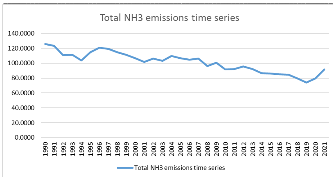
Figure 14. Total NH 3 emissions time series from 1990 to 2021.
