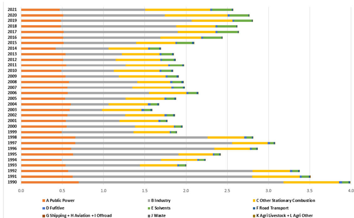
Figure 41. Distribution of Cd between sectors for period 1990 – 2021
