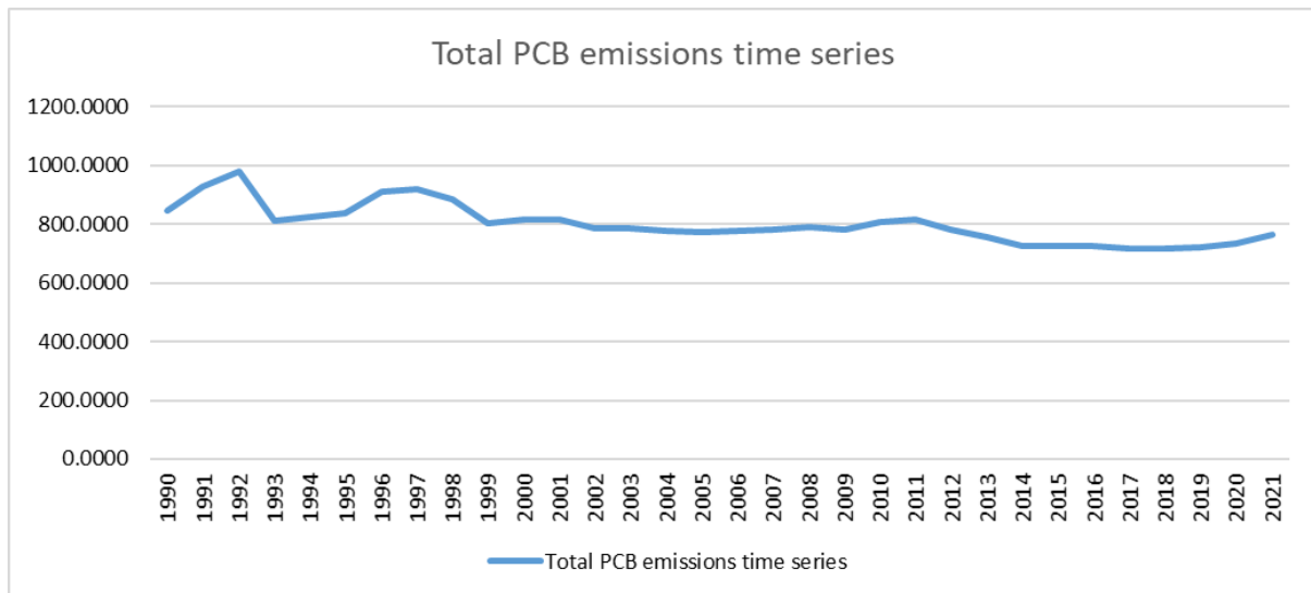
Figure 102.Total PCB emissions time series from 1990 to 2021.
