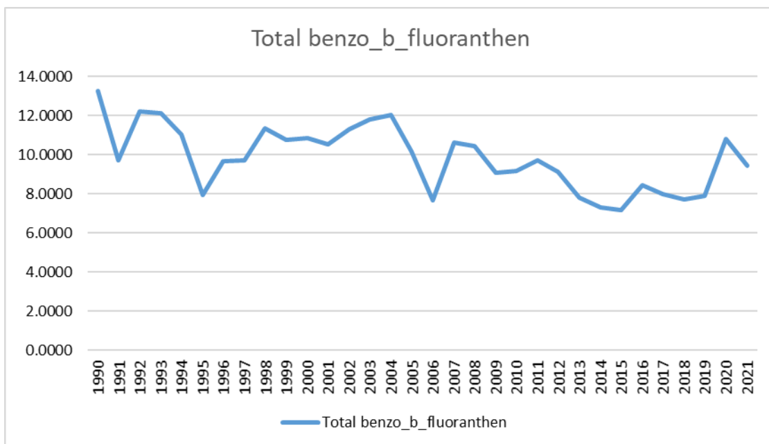
Figure 82. Total benzo b fluoranthene emissions time series from 1990 to 2021.
