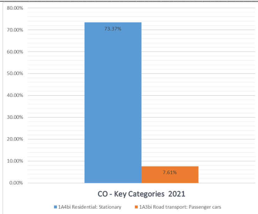
Figure 35. Key Categories assessments of CO emissions for 2021.
