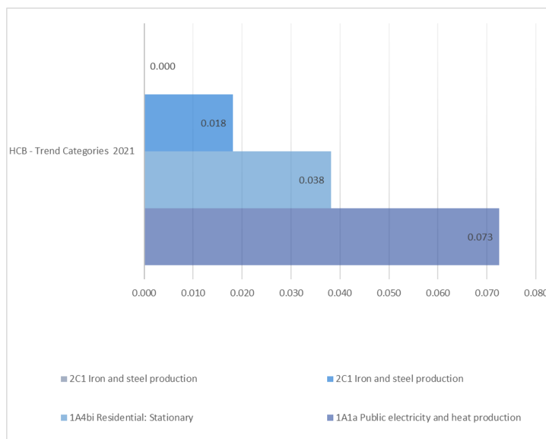
Figure 100. Trends assessments of HCB emissions for base year and 2021
