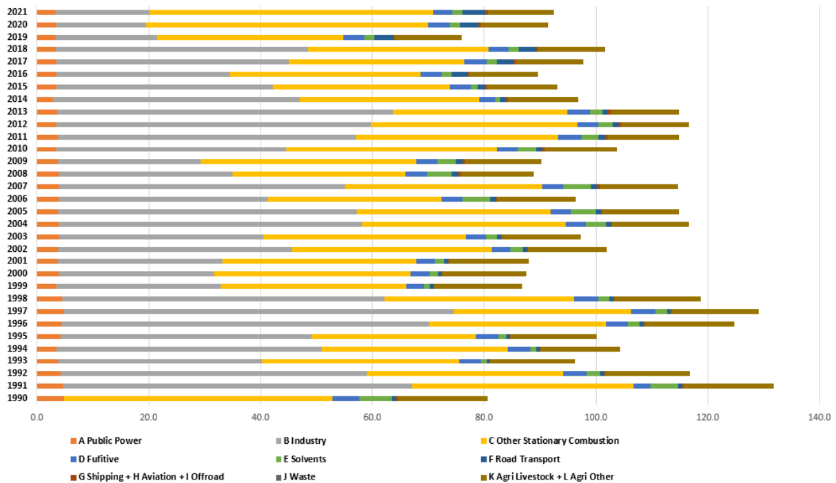
Figure 25. Distribution of TSP between sectors for period 1990 – 2021.
