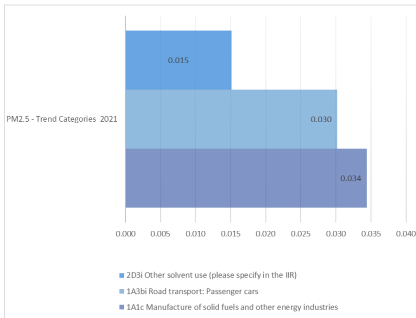
Figure 20. Trends assessments of PM 2.5 emissions for base year and 2021
