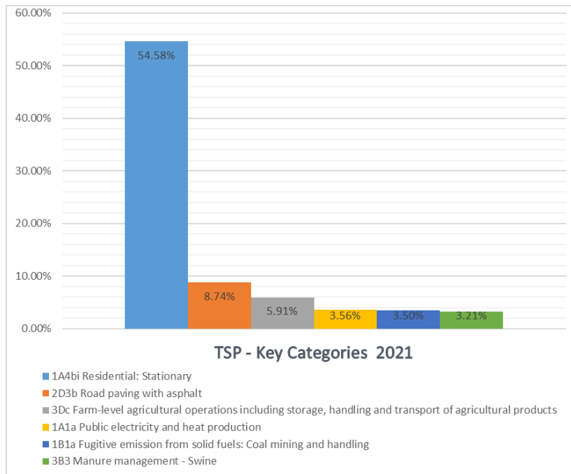
Figure 27. Key Categories assessments of TSP emissions for 2021
