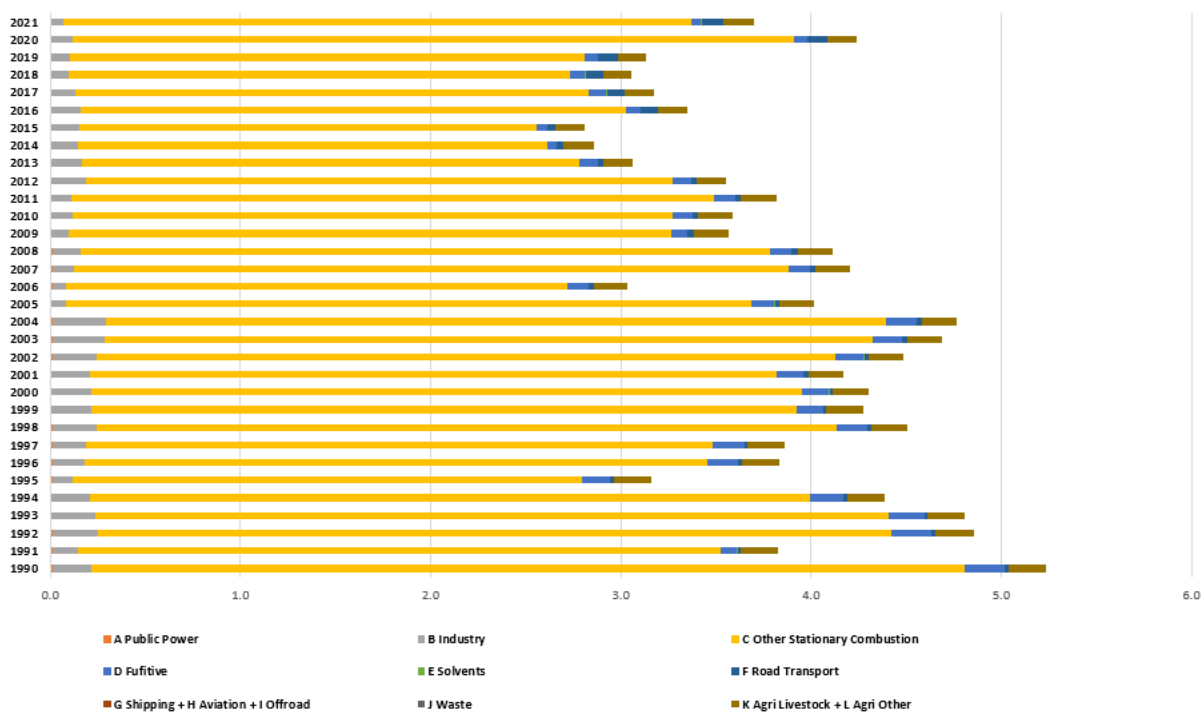
Figure 85. Distribution of benzo (k) fluoranthene between sectors for period 1990 – 2021.
