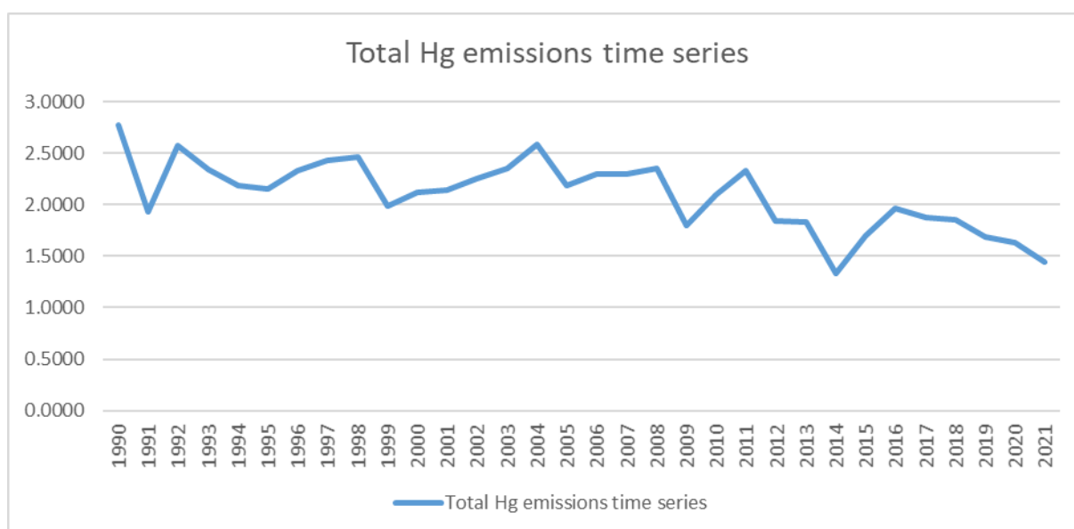
Figure 46. Total Hg emissions time series from 1990 to 2021.
