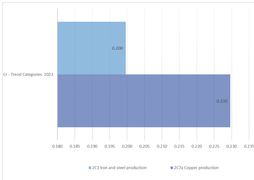
Figure 56. Trends assessments of Cr emissions for base year and 2021
