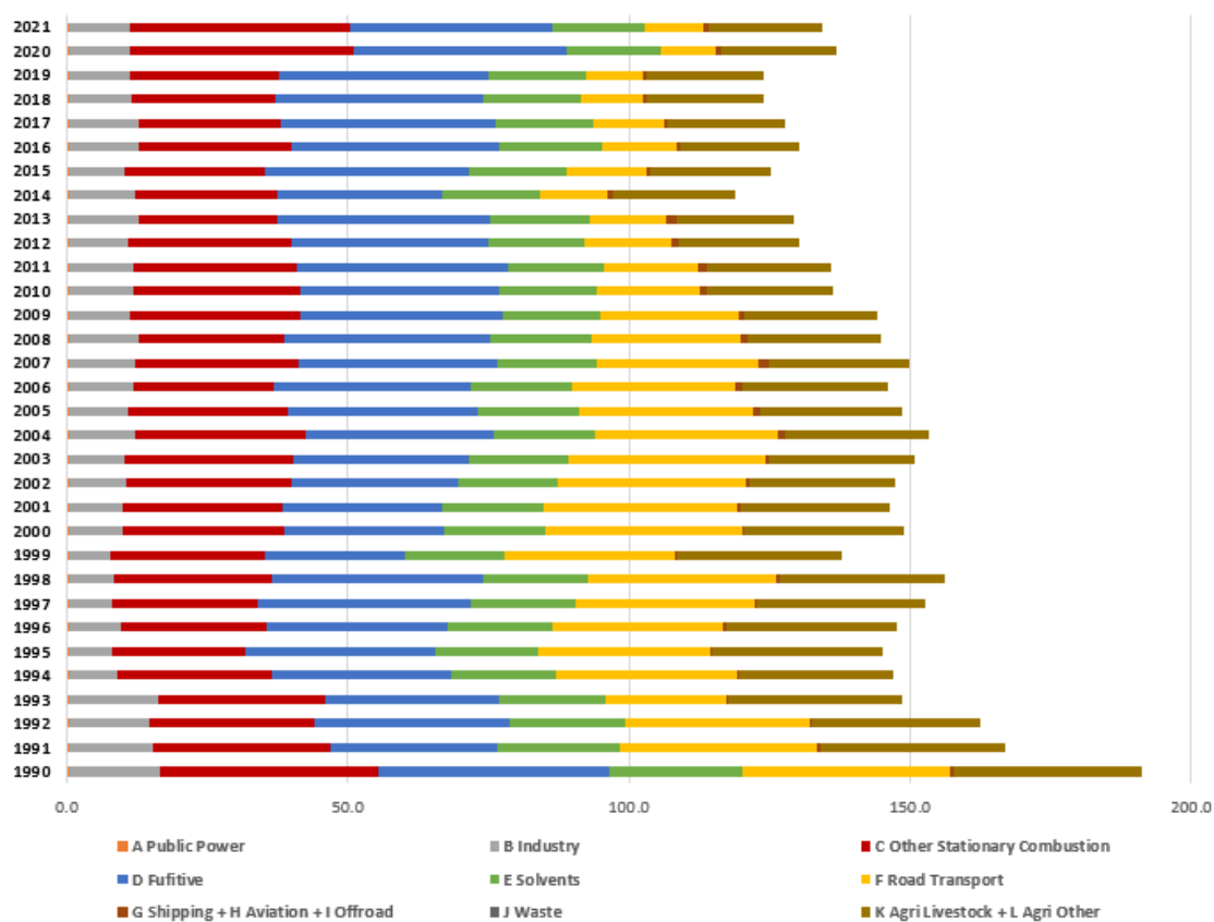
Figure 5. Distribution of NMVOC between sectors for period 1990 – 2021
