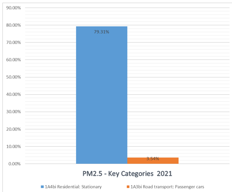
Figure 19. Key Categories assessments of PM 2.5 emissions for 2021.
