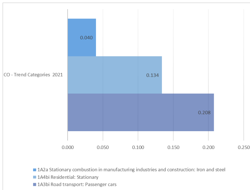
Figure 36. Trends assessments of CO emissions for base year and 2021
