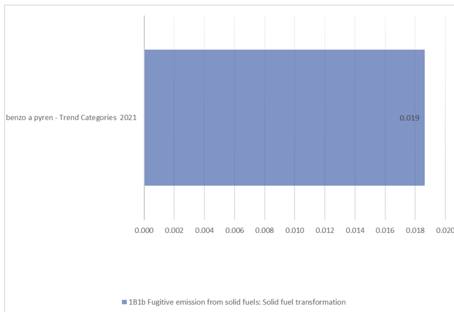
Figure 80. Trends assessments of Benzo a pyren emissions for base year and 2021
