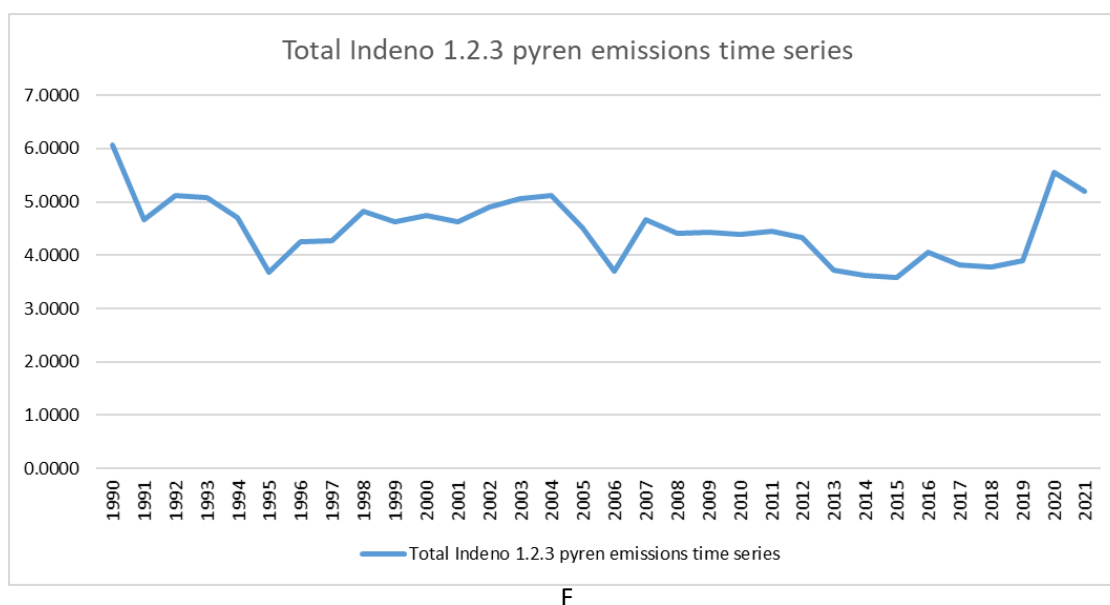
Figure 90. Total Indeno 1,2,3 pyren emissions time series from 1990 to 2021.
