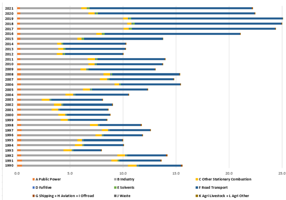
Figure 57. Distribution of Cu between sectors for period 1990 – 2021.
