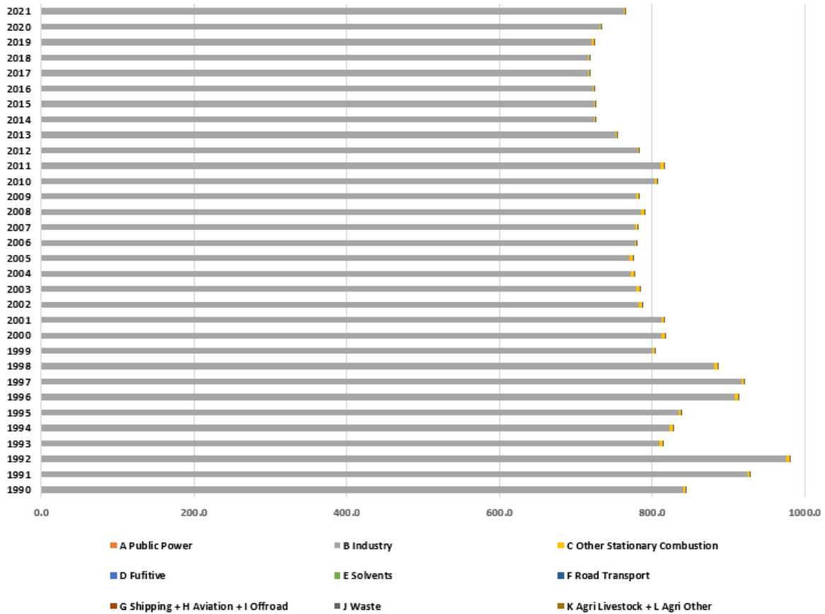
Figure 101. Distribution of PCB between sectors for period 1990 – 2021.
