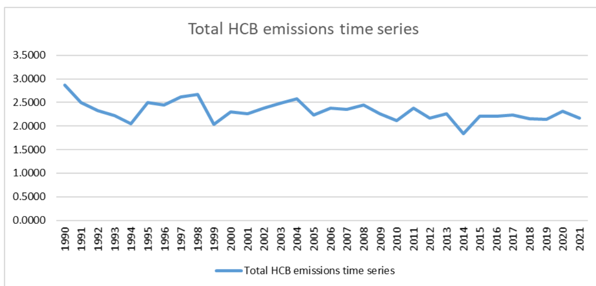
Figure 98.Total HCB emissions time series from 1990 to 2021.
