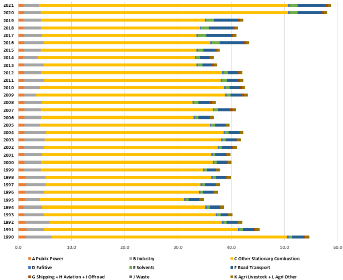
Figure 17. Distribution of PM2.5 between sectors for period 1990 – 2021
