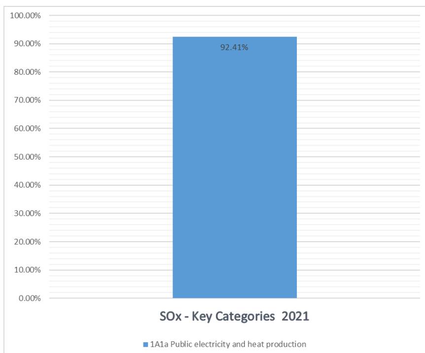
Figure 11. Key Categories assessments of SOx emissions for 2021.
