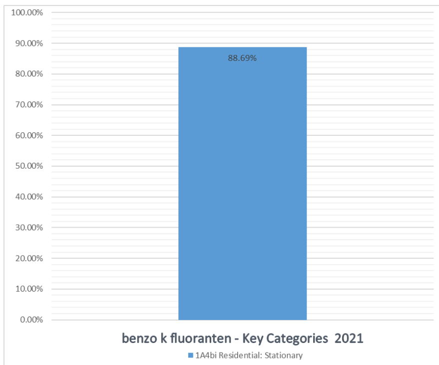
Figure 87. Key Categories assessments of benzo k fluoranthen emissions for 2021.
