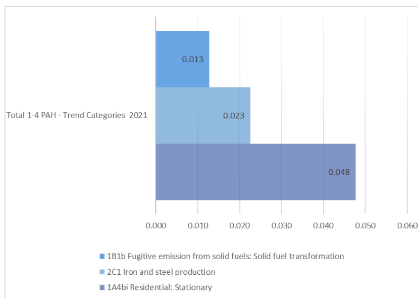
Figure 96. Trends assessments of Total 1-4 PAH emissions for base year and 2021
