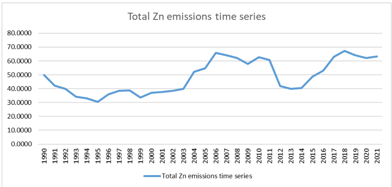
Figure 70. Total Zn emissions time series from 1990 to 2021.
