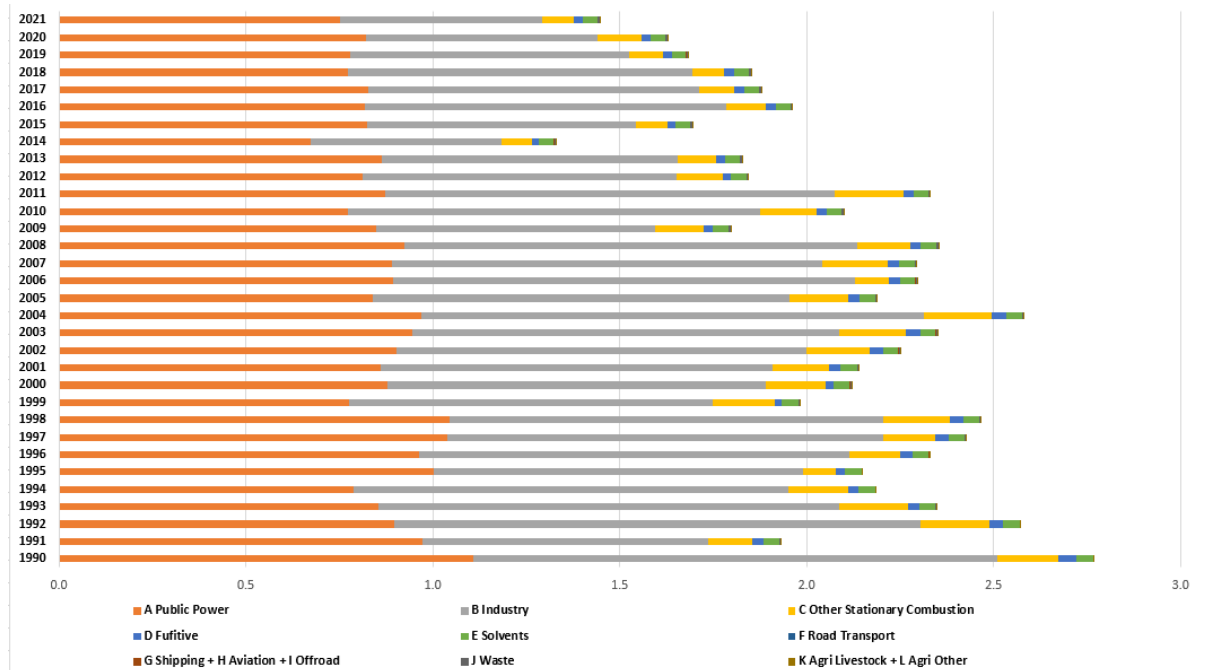
Figure 45. Distribution of Hg between sectors for period 1990 – 2021
