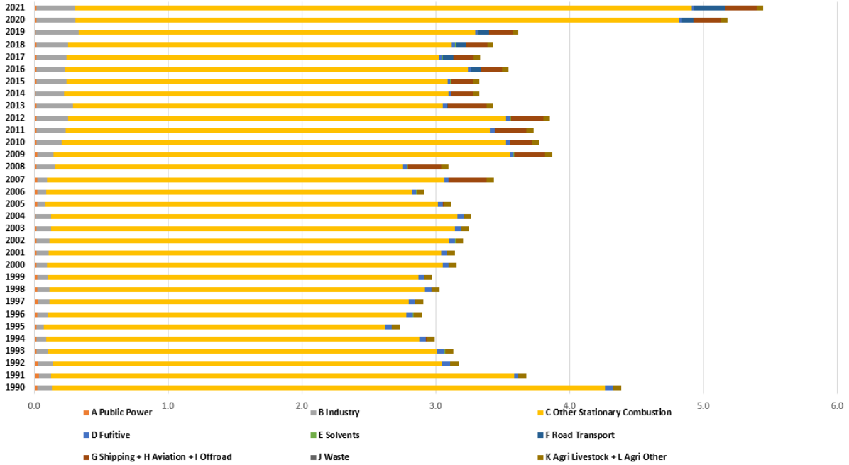
Figure 29. Distribution of BC between sectors for period 1990 – 2021.
