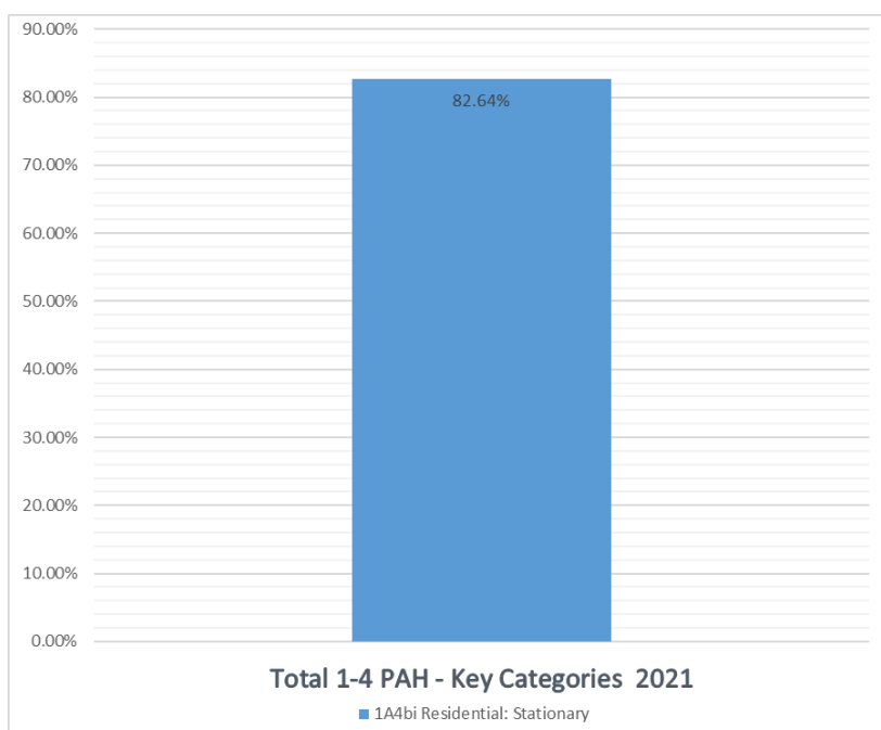
Figure 95. Key Categories assessments of Total 1-4 PAH emissions for 2021.
