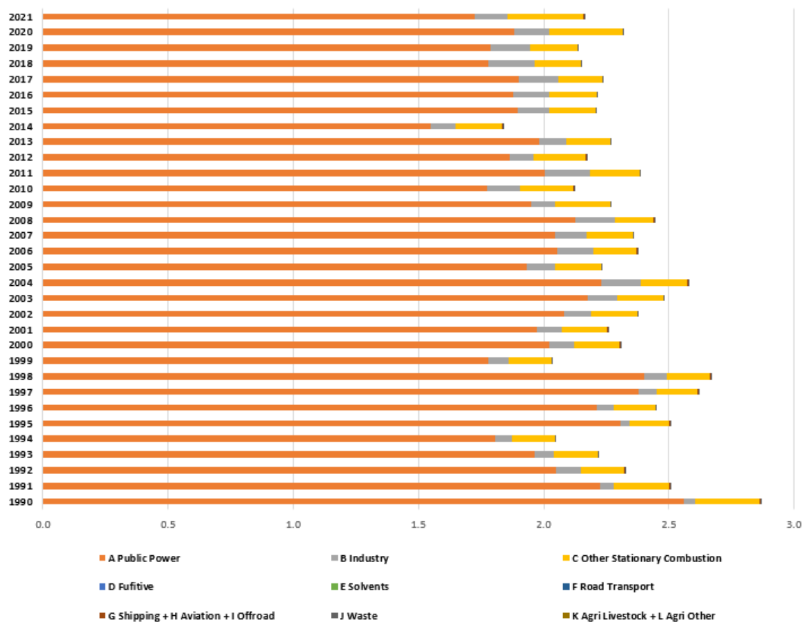
Figure 97. Distribution of HCB between sectors for period 1990 – 2021.
