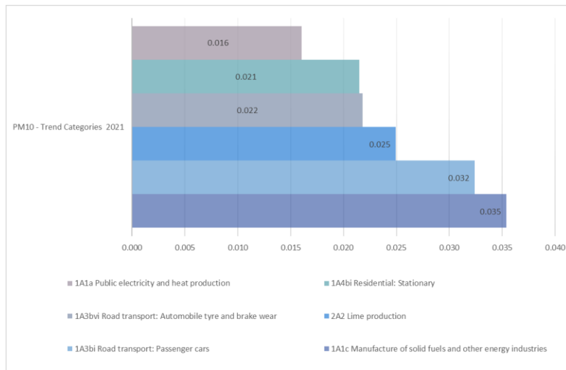
Figure 24. Trends assessments of PM10 emissions for base year and 2021
