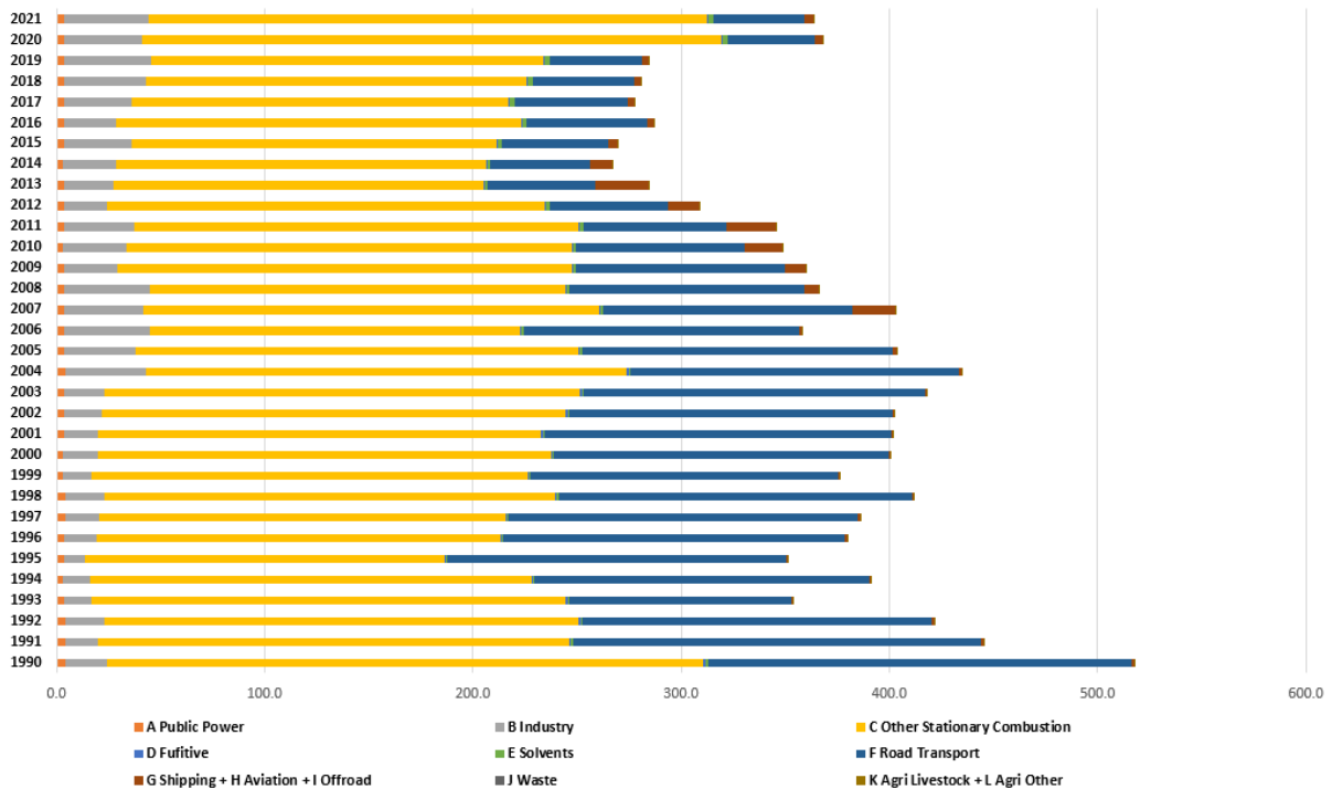
Figure 33. Distribution of CO between sectors for period 1990 – 2021
