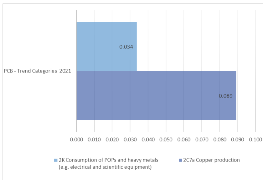
Figure 104. Trends assessments of PCB emissions for base year and 2021
