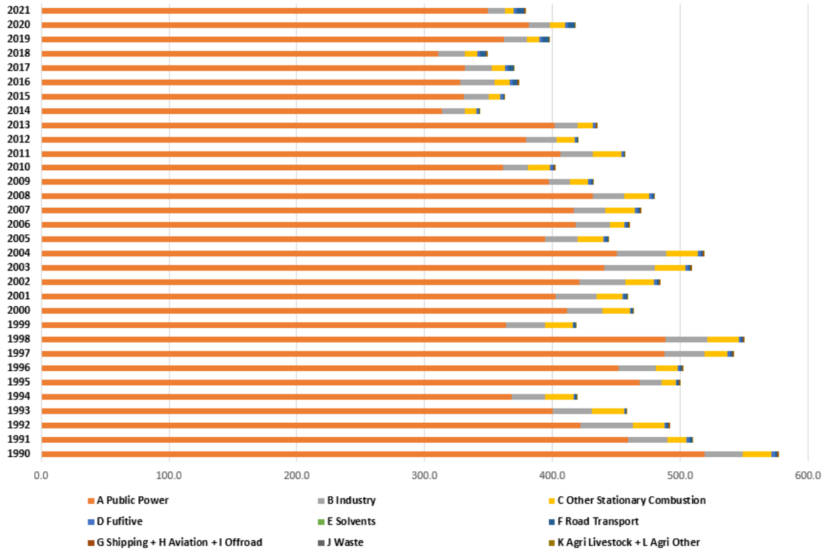
Figure 9. Distribution of SOx between sectors for period 1990 – 2021
