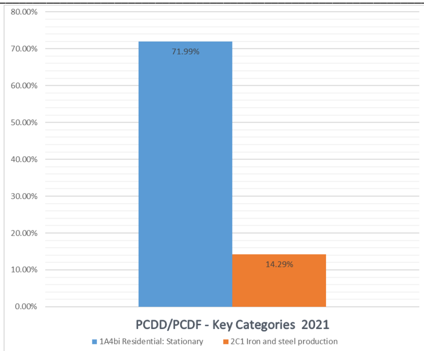
Figure 75. Key Categories assessments of PCDD/PCDF emissions for 2021.
