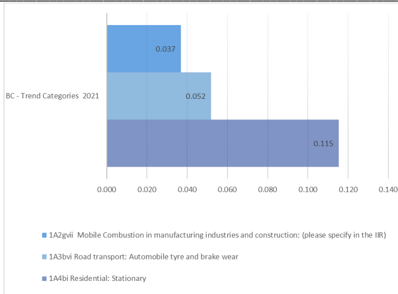
Figure 32. Trends assessments of BC emissions for base year and 2021
