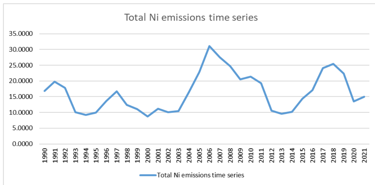
Figure 62. Total Ni emissions time series from 1990 to 2021.
