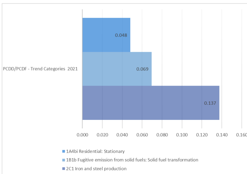
Figure 76. Trends assessments of PCDD/PCDF emissions for base year and 2021
