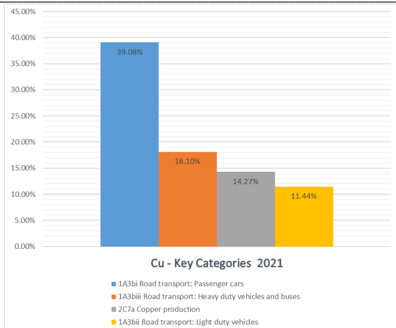
Figure 59. Key Categories assessments of Cu emissions for 2021
