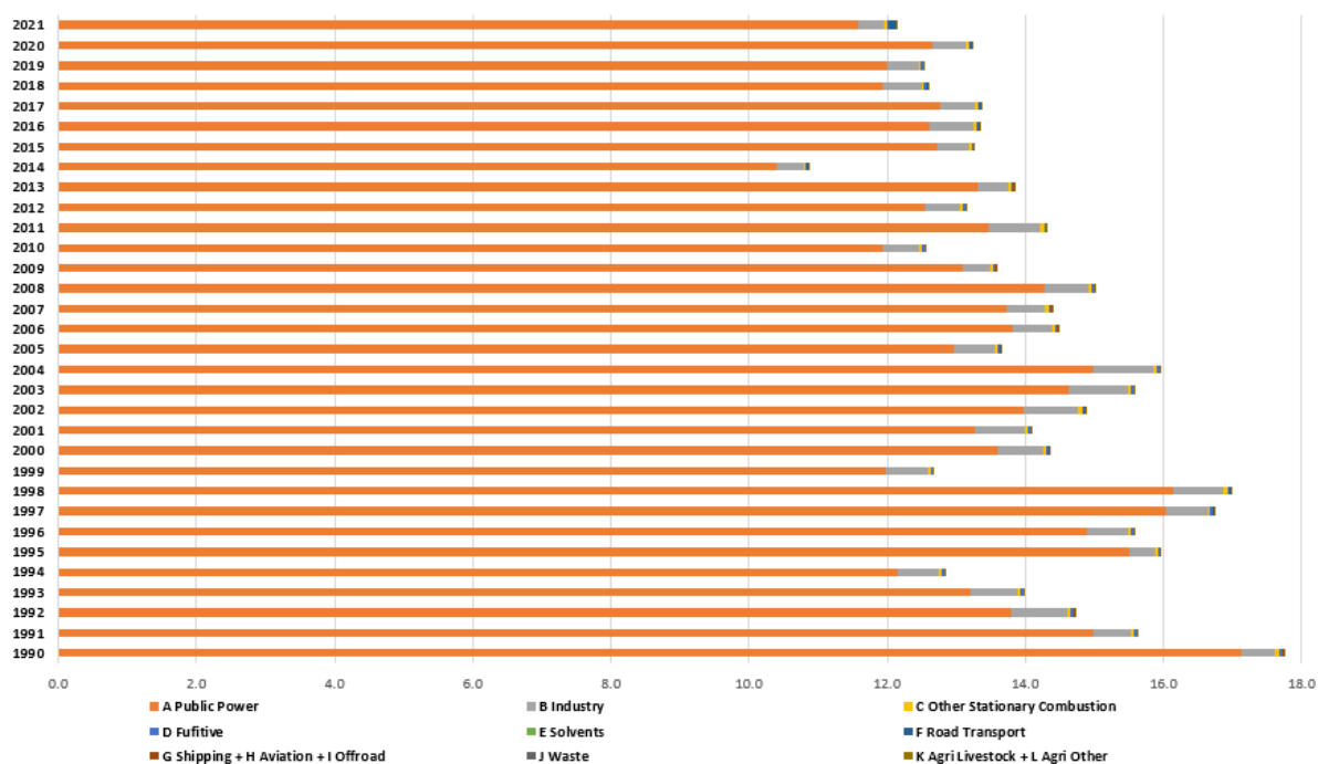
Figure 65. Distribution of Se between sectors for period 1990 – 2021.
