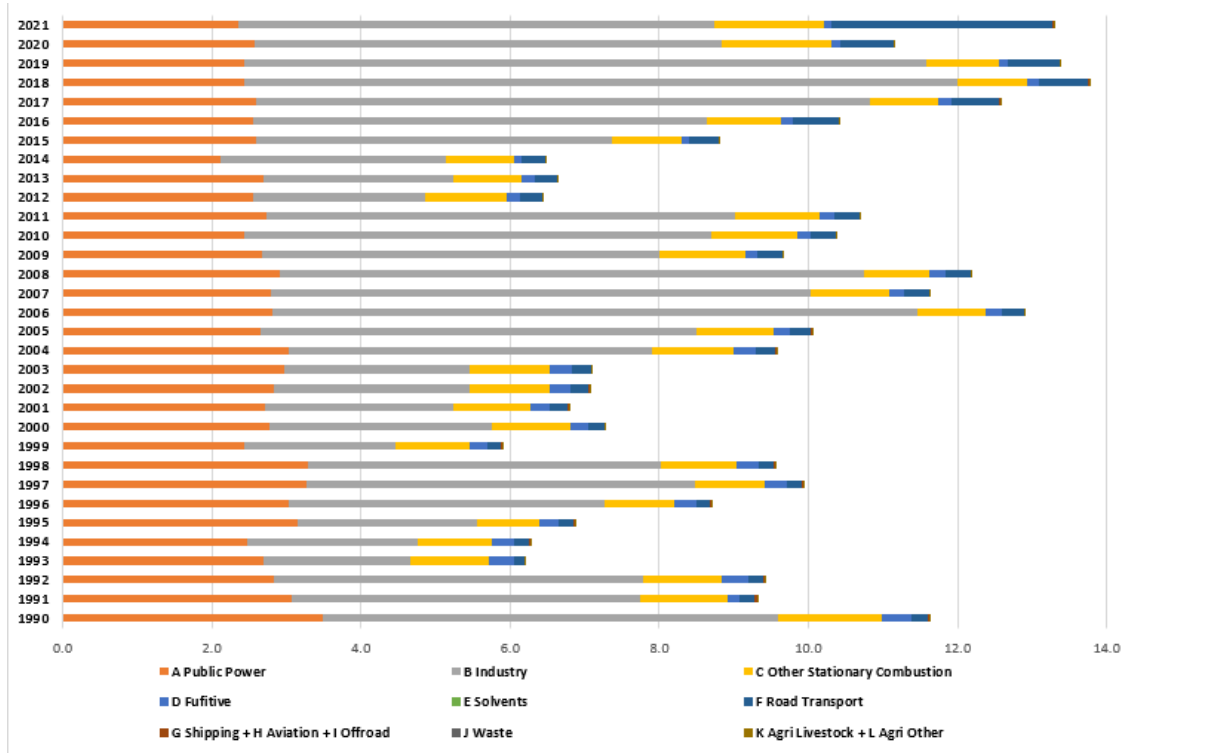
Figure 53. Distribution of Cr between sectors for period 1990 – 2021.
