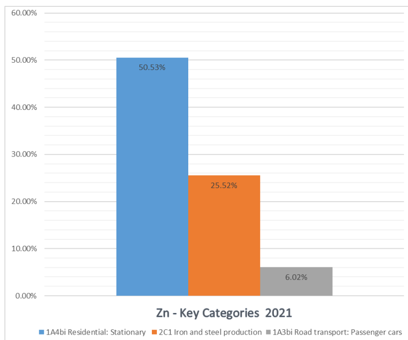
Figure 71. Key Categories assessments of Zn emissions for 2021
